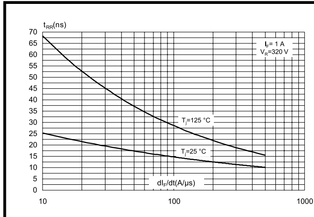
Figure 7: Reverse recovery time versus dI_F/dt (typical values)
