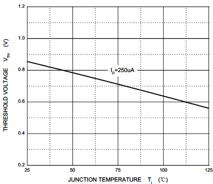
Threshold Voltage
