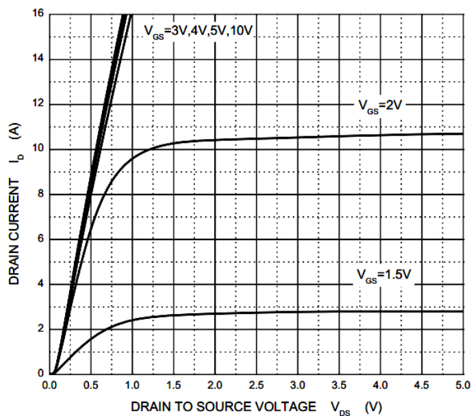
Output Characteristics
