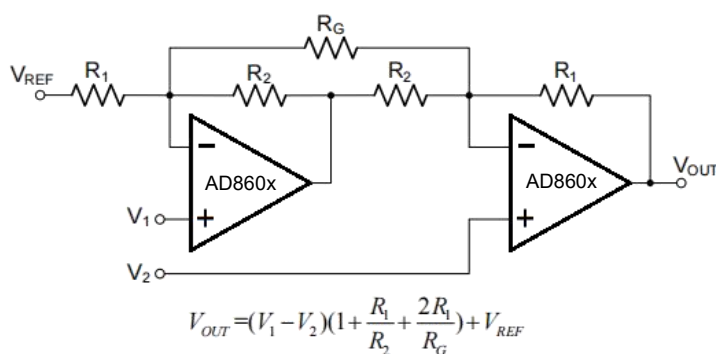
Figure 9. Instrumentation Amplifier
