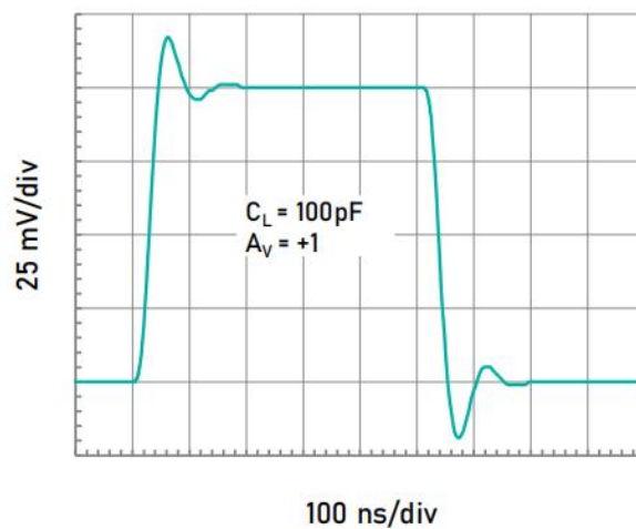
Small Signal Step Response (500 mV).
