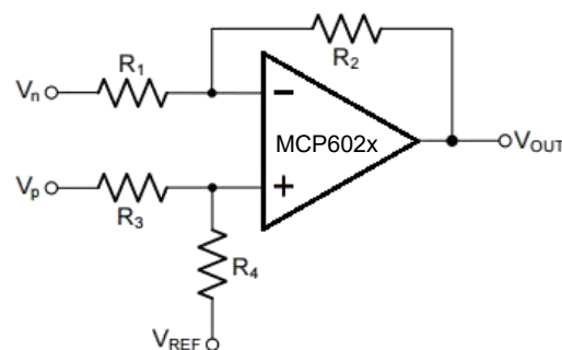
Figure 8. Differential Amplifier
