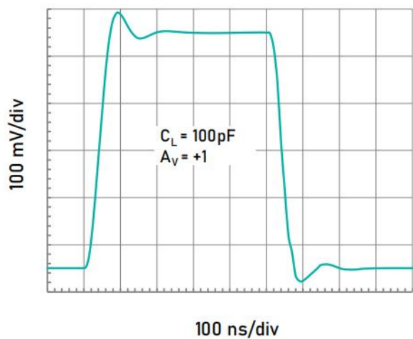
Small Signal Step Response (500 mV).
