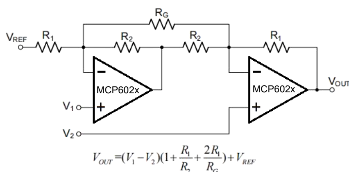
Figure 9. Instrumentation Amplifier
