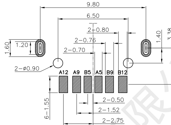
RECOMMENDER P.C.B LAYOUT TOP VIEW (GENERAL TOLERANCE ±0.05)
