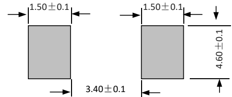
Recommended Pad Layout (mm)
