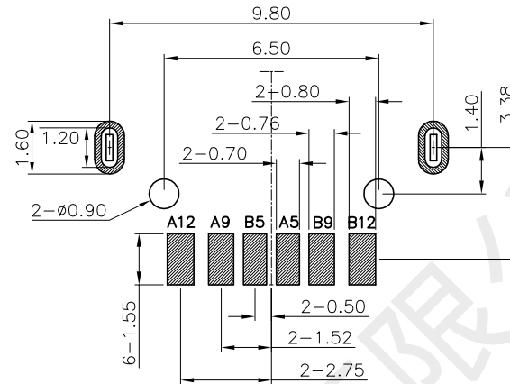
RECOMMENDER P.C.B LAYOUT TOP VIEW (GENERAL TOLERANCE ±0.05)
