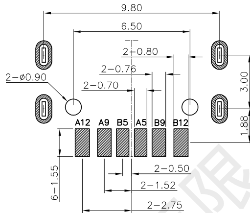
RECOMMENDER P.C.B LAYOUT TOP VIEW (GENERAL TOLERANCE ±0.05)
