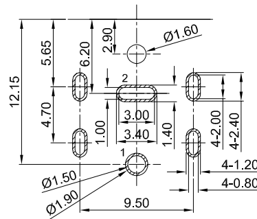
PCB REFERENCE DIAGRAM TOLERANCE: ±0.05
