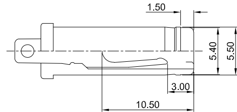
MATING PLUG Ø5.5xØ2.5mm
