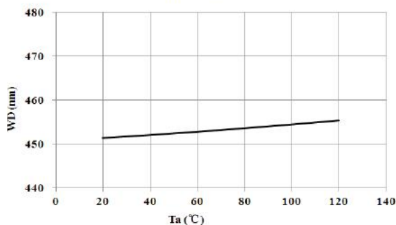
Fig.5- Dominant Wavelength (@350mA) vs. Ambient Temperature
