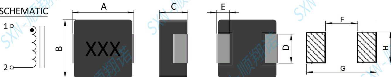
Recommended Land Pattern
