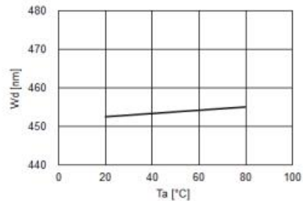
Fig.5 – Dominant Wavelength (@350mA) vs. Ambient Temperature
