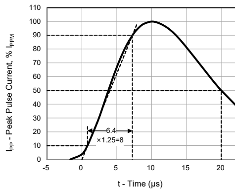
Fig.3 - 8/20 \mu\text{s} Pulse Waveform
