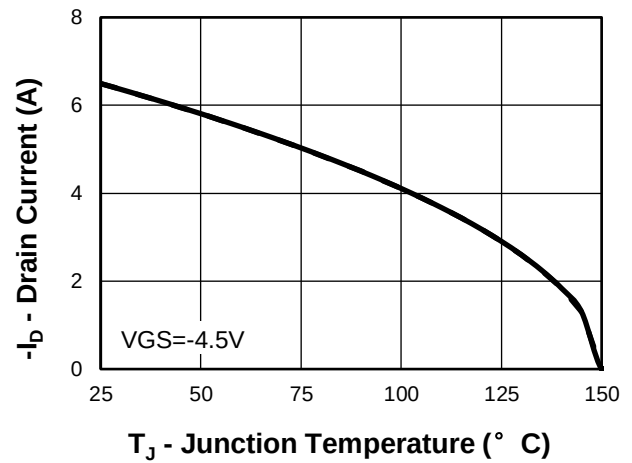
Fig 2. Drain Current
