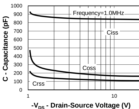
Fig 10. Capacitance Characteristics
