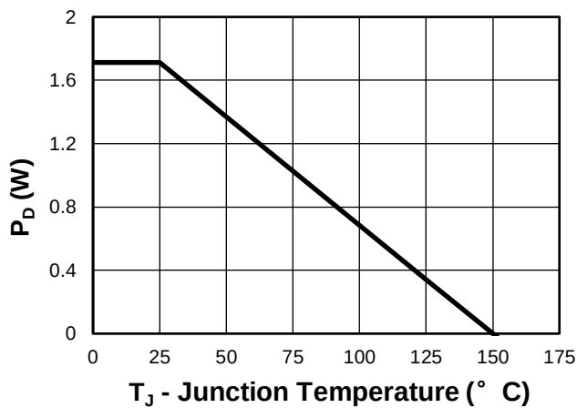
Fig 3. Power Dissipation
