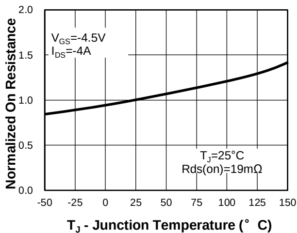
Fig 8. Rdson vs. Junction Tem Characteristics
