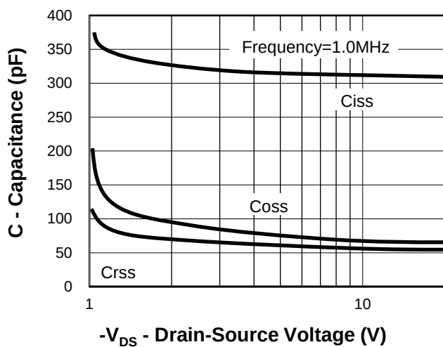
Fig 10. Capacitance Characteristics
