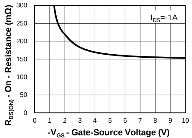
Fig 7. Gate-Source on Resistance
