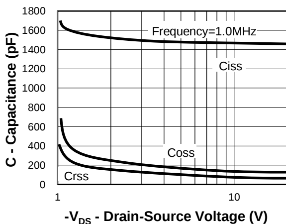
Fig 10. Capacitance Characteristics
