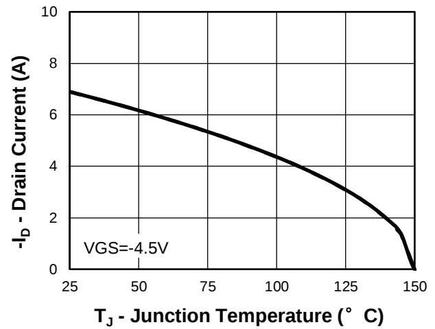
Fig 2. Drain Current
