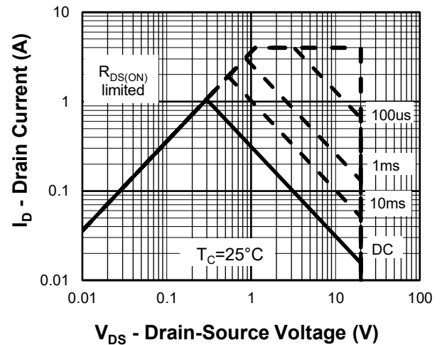
Fig 4. Safe Operation Area(SOA)
