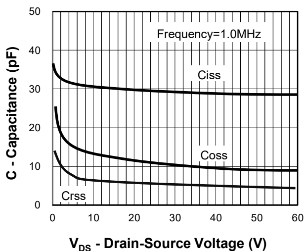
Fig 10. Capacitance Characteristics
