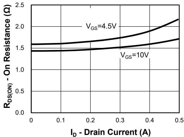
Fig 6. Rdson vs. Drain Current Characteristics
