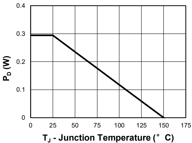
Fig 3. Power Dissipation
