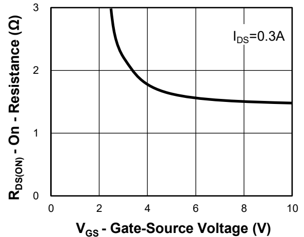
Fig 7. Gate-Source on Resistance
