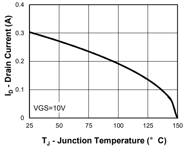
Fig 2. Drain Current
