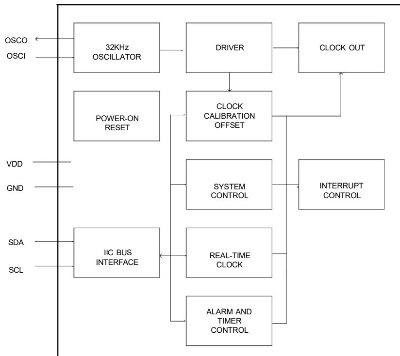
Figure1 Function block
