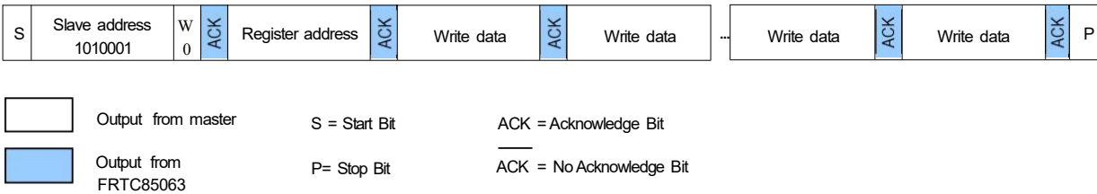
Figure10 Write Mode Sequence
