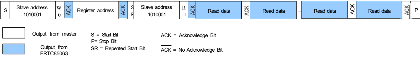
Figure9 Read Mode Sequence
