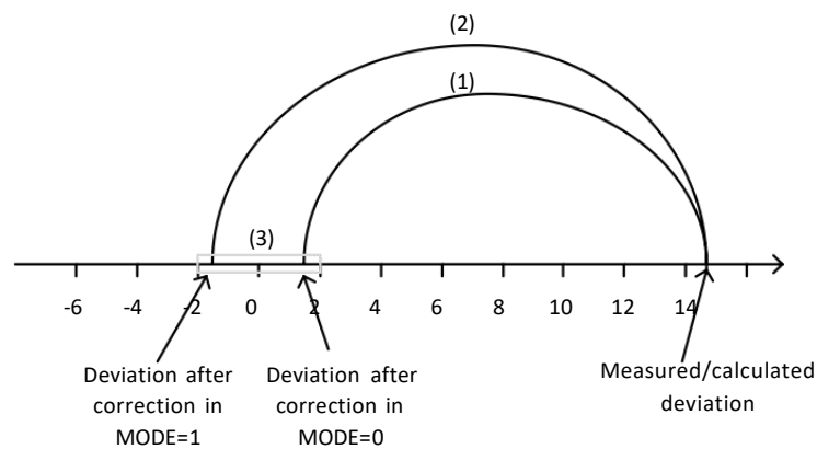
Figure5 Offset calibration calculation workflow
