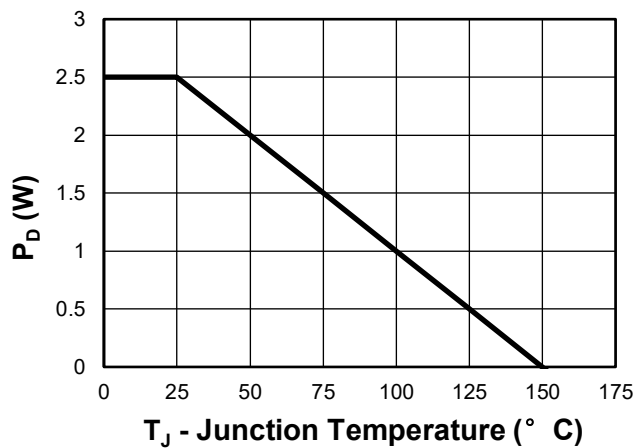
Fig 3. Power Dissipation
