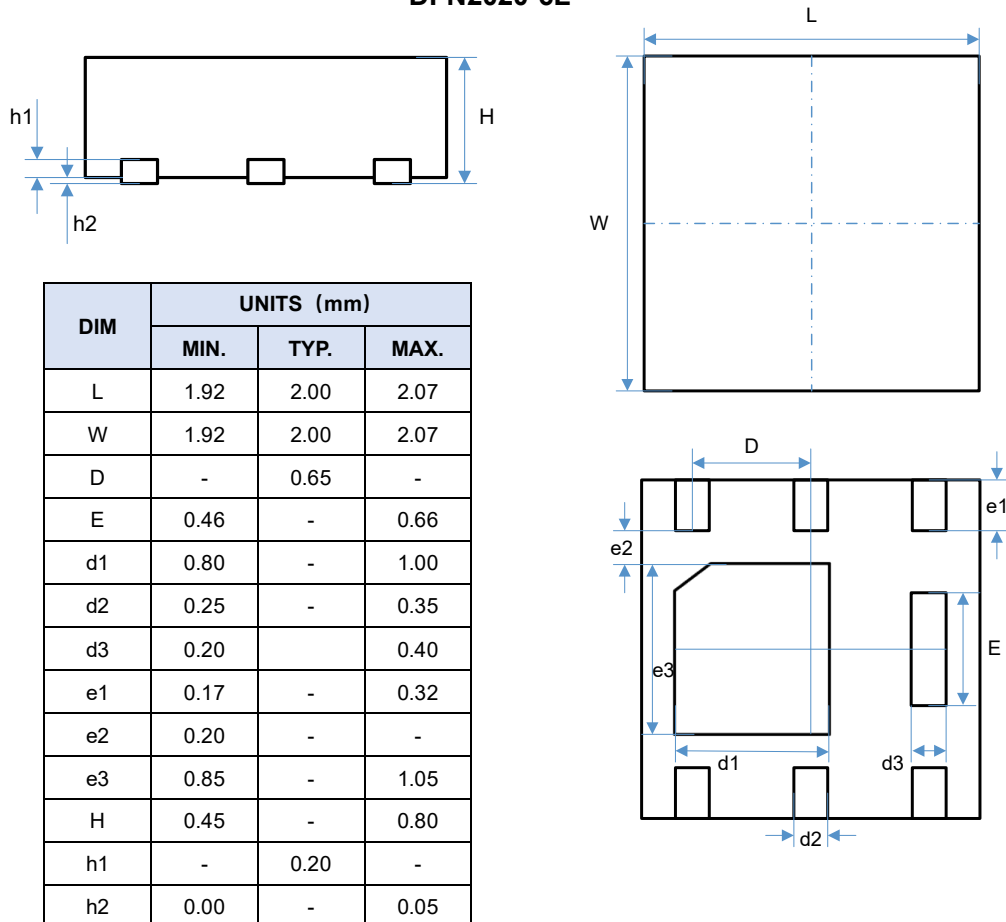
DFN2020-6L
