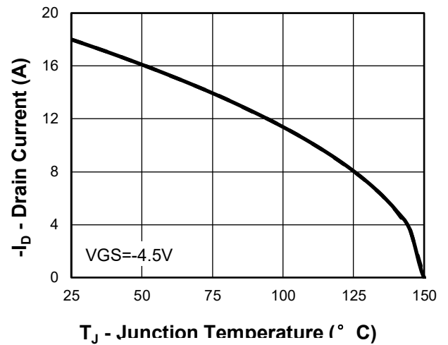
Fig 2. Drain Current
