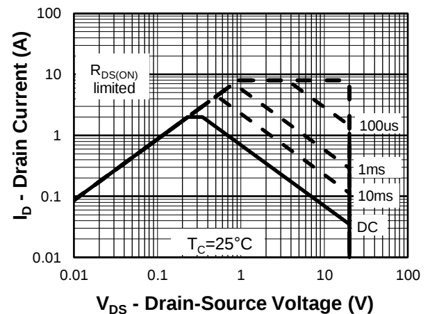
Fig 4. Safe Operation Area(SOA)
