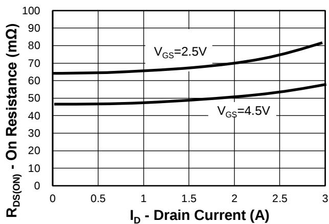
Fig 6. Rdson vs. Drain Current Characteristics
