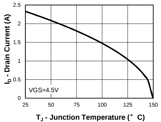
Fig 2. Drain Current
