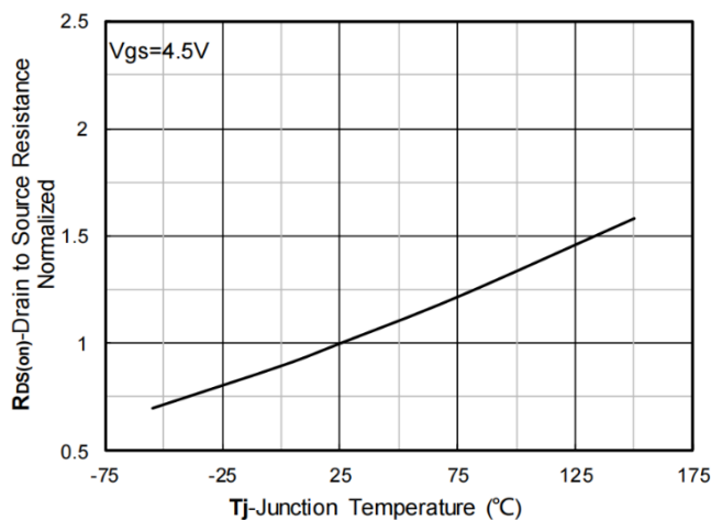
Fig 6: Normalized On-Resistance
