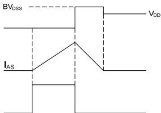
Fig10 EAS Waveform
