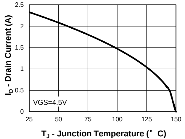
Fig 2. Drain Current
