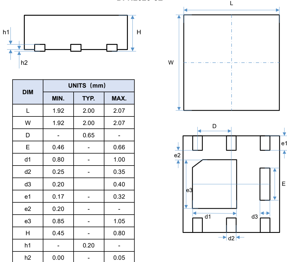
DFN2020-6L
