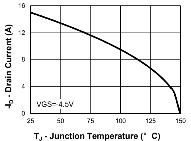
Fig 2. Drain Current
