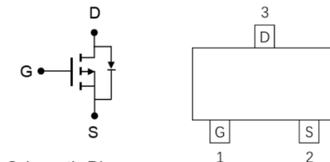
Schematic Diagram
