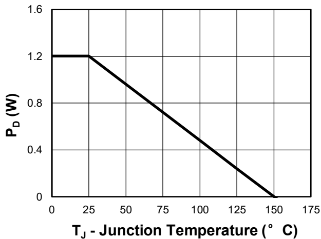
Fig 3. Power Dissipation
