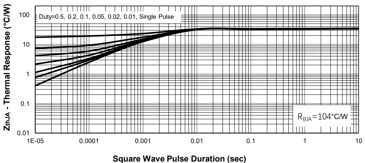
Fig 5. Thermal Transient Impedance
