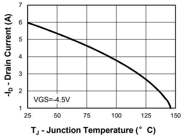
Fig 2. Drain Current
