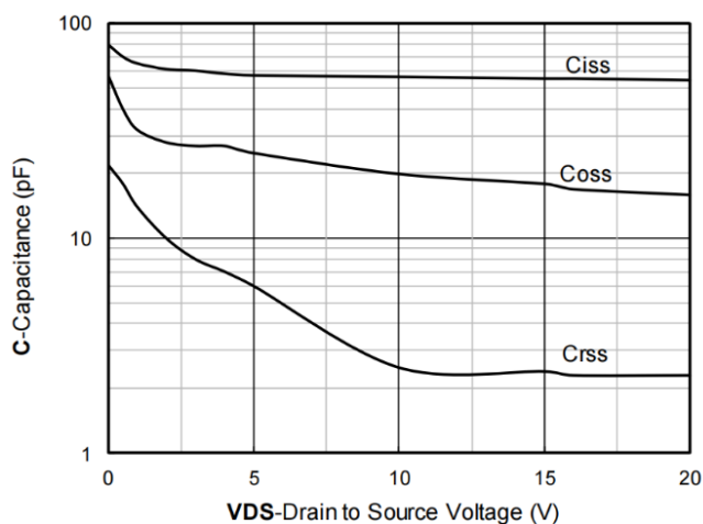
Fig 3. Capacitance Characteristics
