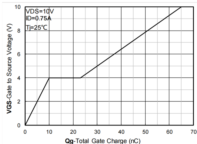
Fig 4. Gate Charge
