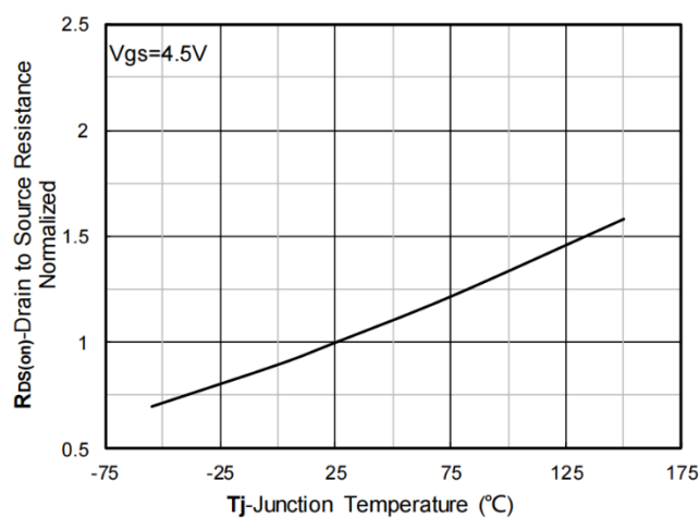
Fig 6. Normalized On-Resistance
