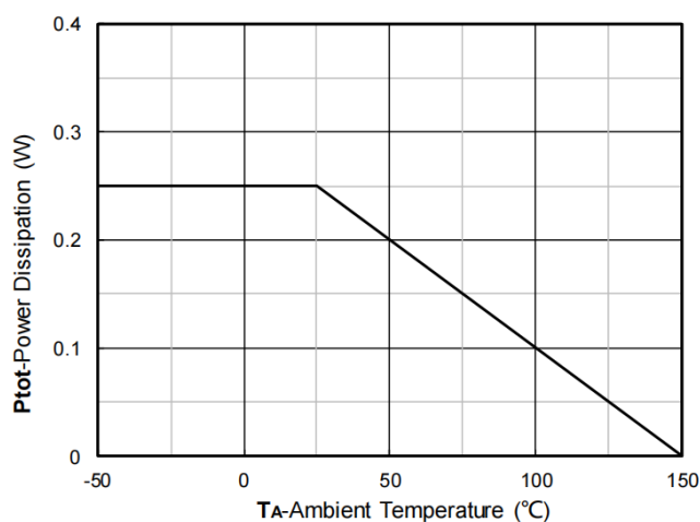
Fig 12. Power dissipation
