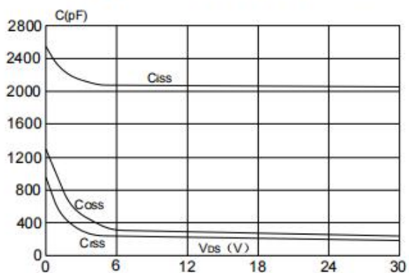
Fig5 Capacitance Characteristics
