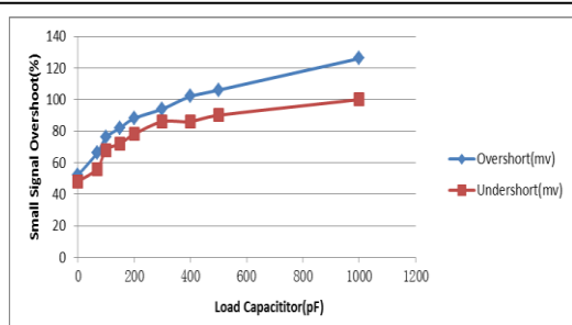
Overshoot (OS) vs Load Capacitance
