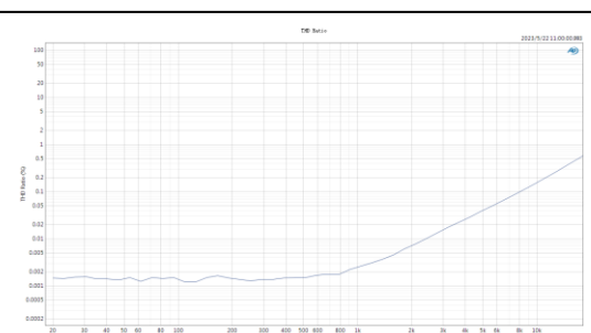
THD vs Frequency
