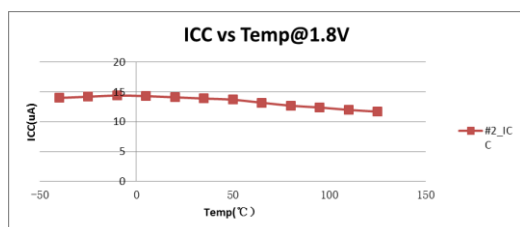
ICC vs Temp
