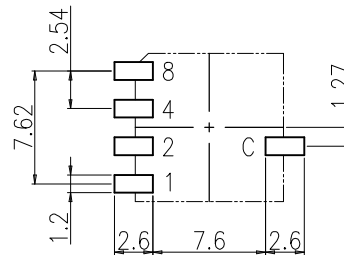
P.C.B DIMENSION (Top View)
