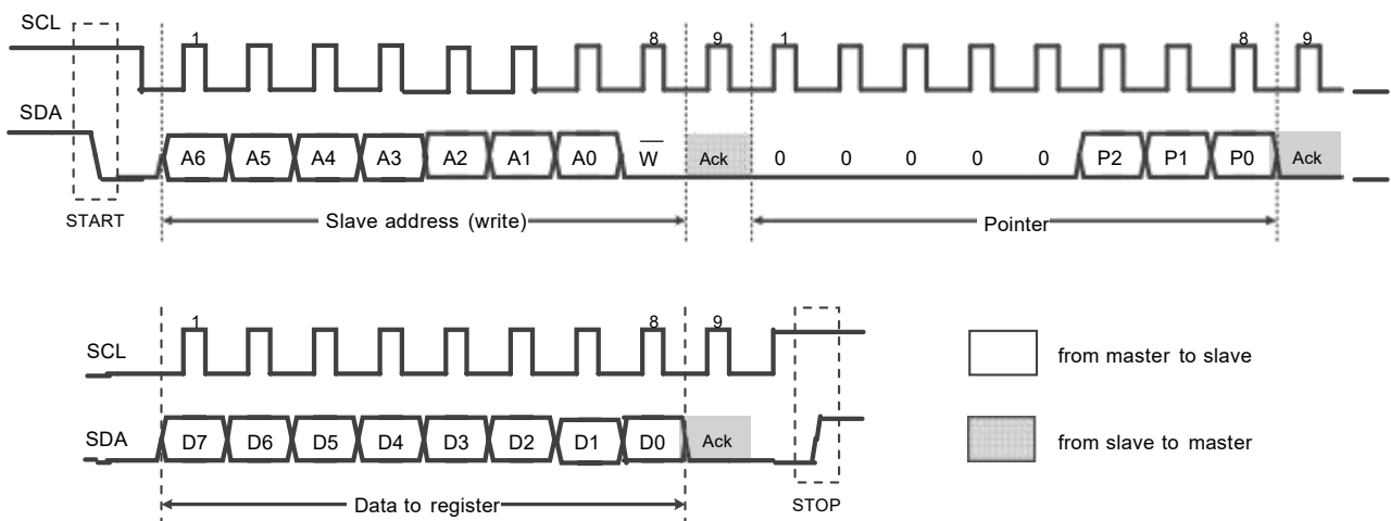
Figure 3. Two-Wire Timing Diagram for Write One Byte
