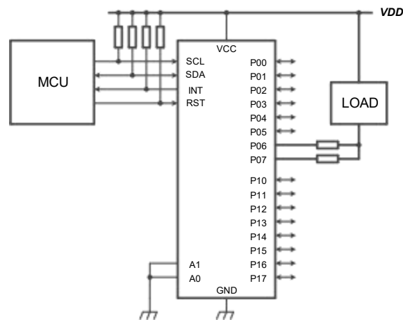
Figure 10. High Current-Drive Load Application
