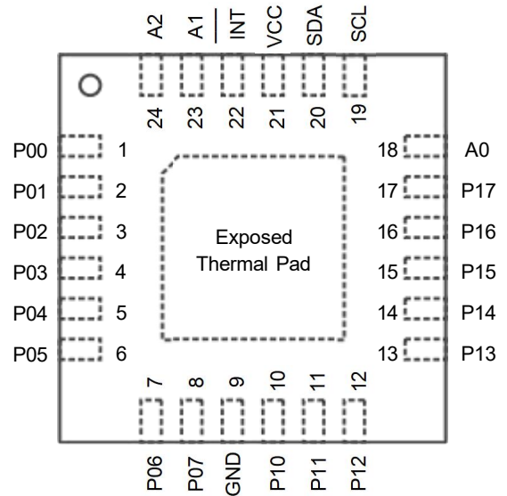
FCA9535Q Top View
