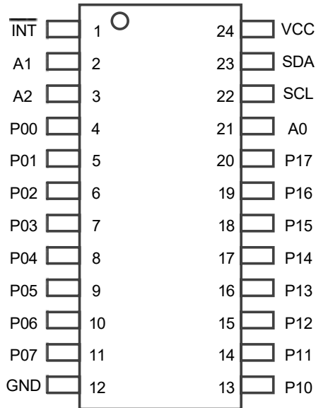
FCA9535T Top View
