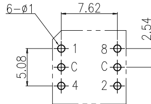
P.C.B DIMENSION (Top View)
