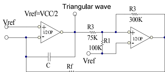
Function Generator
