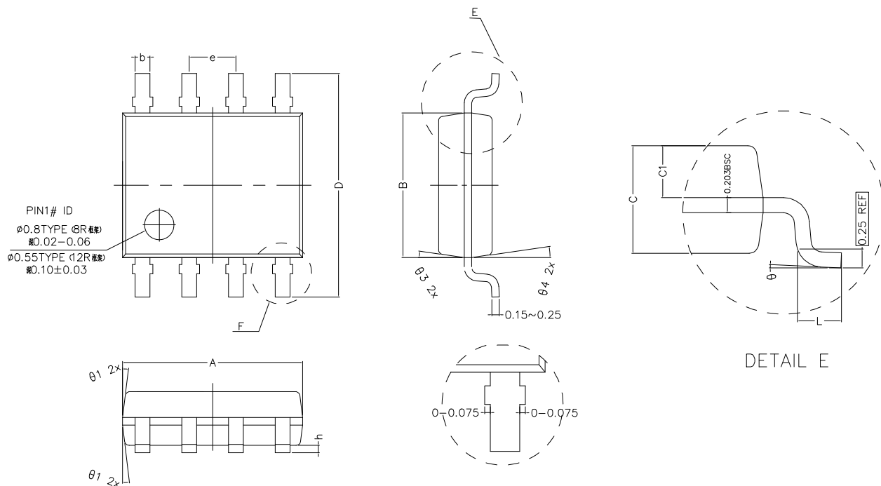
DETAIL F
