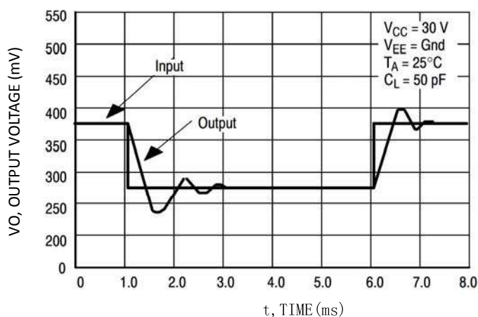
Small Signal Voltage Follower Pulse Response
