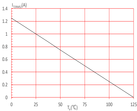
FIG.5: On-state characteristics
