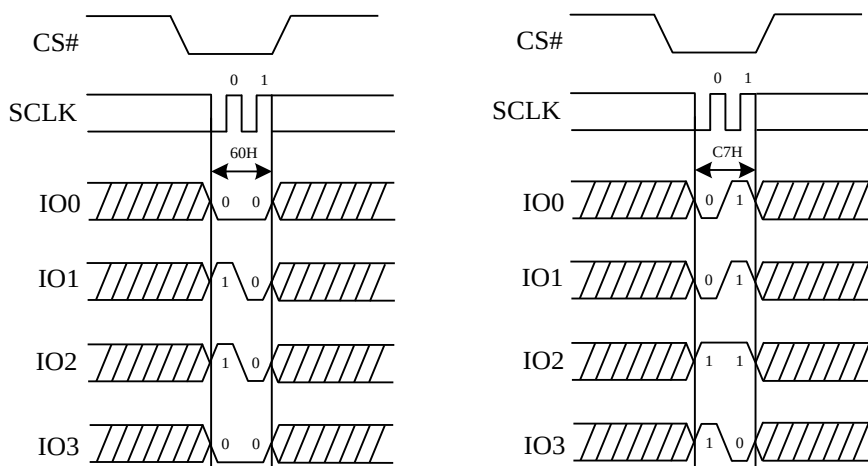
Figure 47. Chip Erase Sequence Diagram (QPI)
