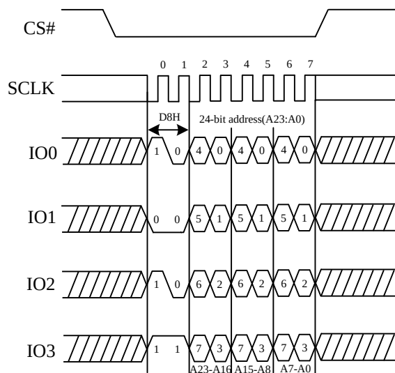
Figure 45. 64KB Block Erase Sequence Diagram (QPI)
