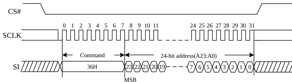
Figure 87. Individual Block/Sector Lock command Sequence Diagram
