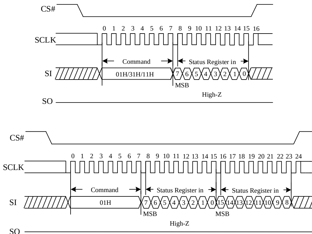
Figure 3. Write Status Register Sequence Diagram
