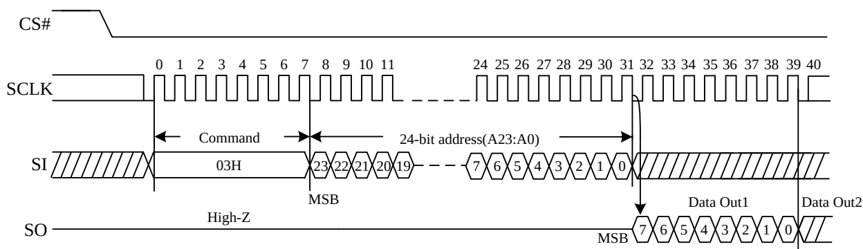
Figure 17. Read Data Bytes Sequence Diagram
