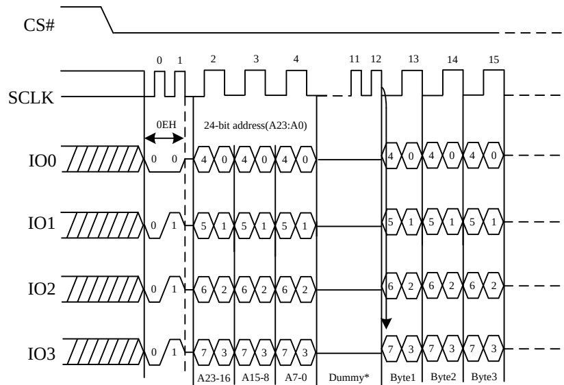
Figure 35. DTR Burst Read With Wrap command Sequence Diagram (QPI)
