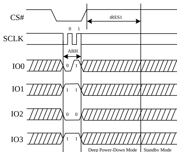
Figure 73. Release Power-Down Sequence Diagram (QPI)
