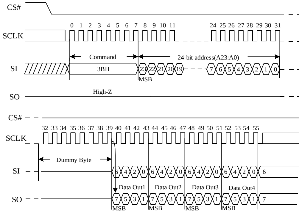
Figure 20. Dual Output Fast Read Sequence Diagram
