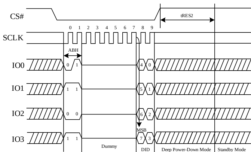
Figure 75. Release Power-Down/Read Device ID Sequence Diagram (QPI)
