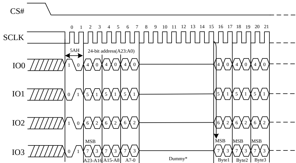
Figure 12. Read Serial Flash Discoverable Parameter command Sequence Diagram (QPI)
