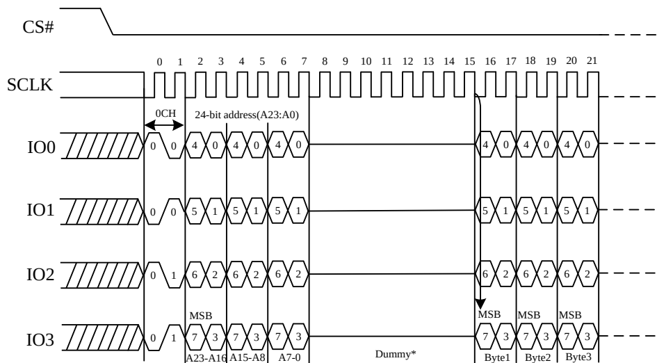
Figure 27. Burst Read with Wrap command Sequence Diagram (QPI)
