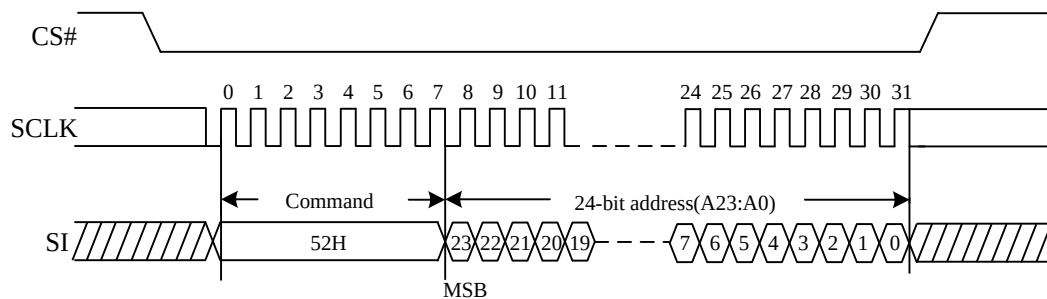
Figure 42. 32KB Block Erase Sequence Diagram
