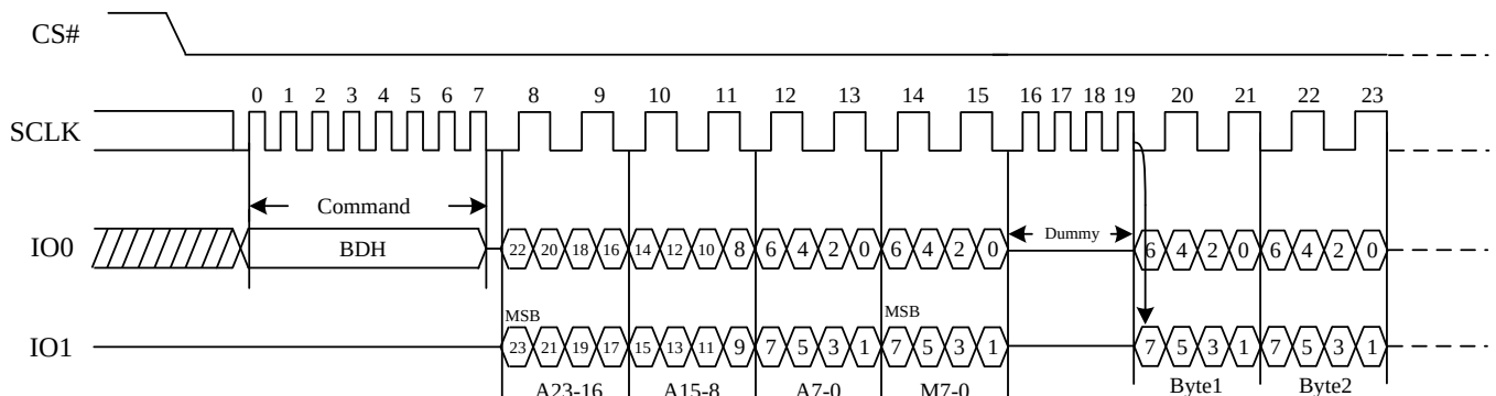
Figure 30. DTR Fast Read Dual I/O(Initial instruction or previous M5-4≠10, SPI Mode only)
