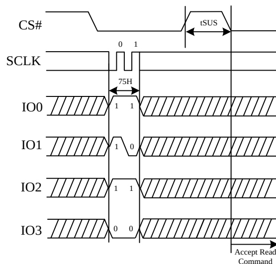
Figure 57. Program/Erase Suspend Sequence Diagram (QPI)
