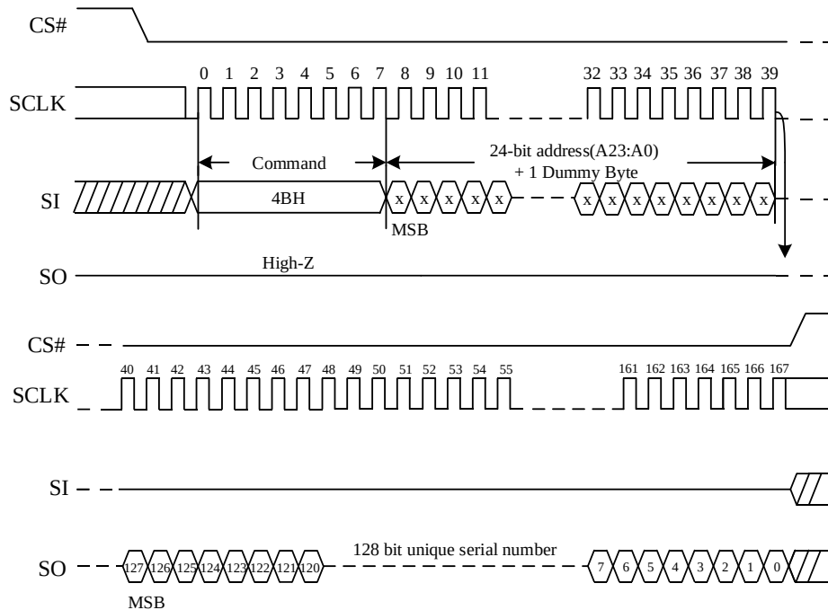
Figure 13. Read Unique ID (RUID) Sequence
