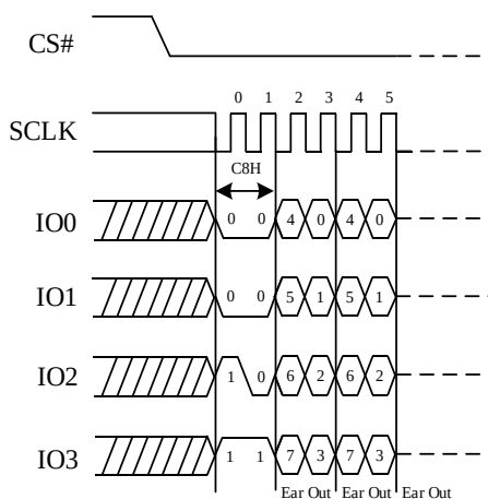
Figure 6. Read Extended Address Register Diagram (QPI)
