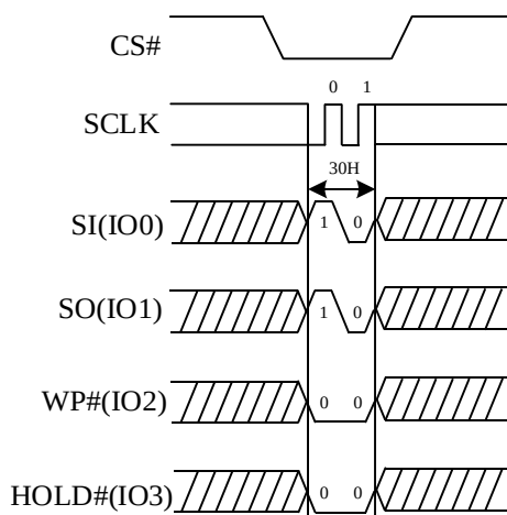
Figure 69. Clear Status Register Flags Sequence Diagram (QPI)
