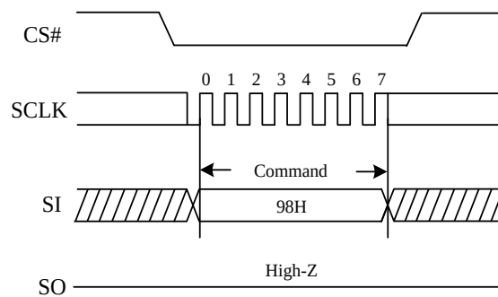
Figure 85. The Global Block/Sector Unlock Sequence Diagram
