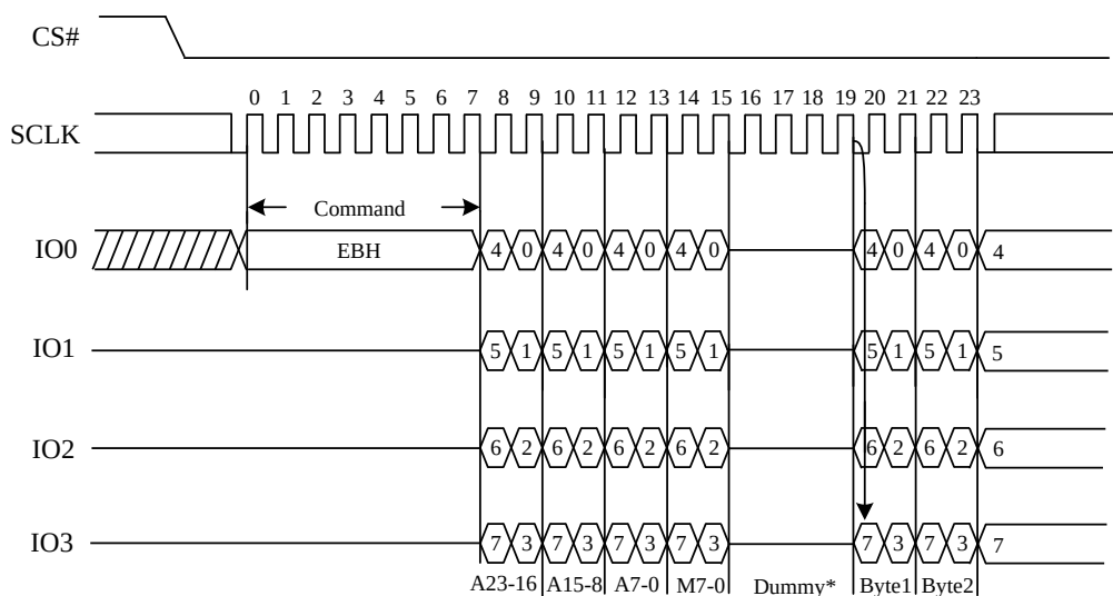
Figure 24. Quad I/O Fast Read Sequence Diagram (M5-4≠(1,0))
