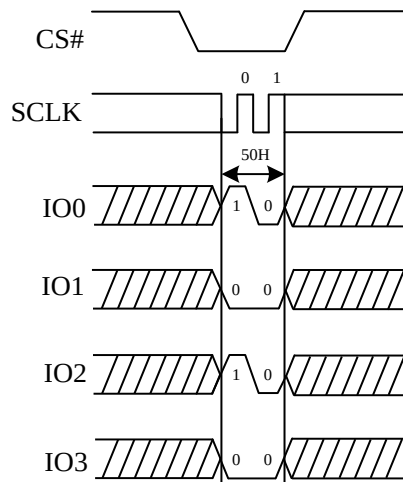
Figure 53. Write Enable for Volatile Status Register Sequence Diagram (QPI)
