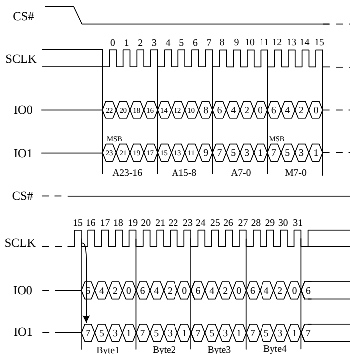
Figure 22. Dual I/O Fast Read Sequence Diagram (M5-4=(1,0))
