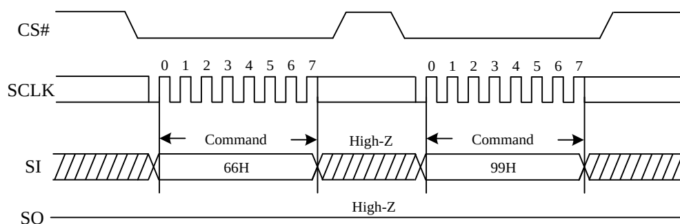
Figure 48. Enable Reset and Reset command Sequence Diagram (SPI)
