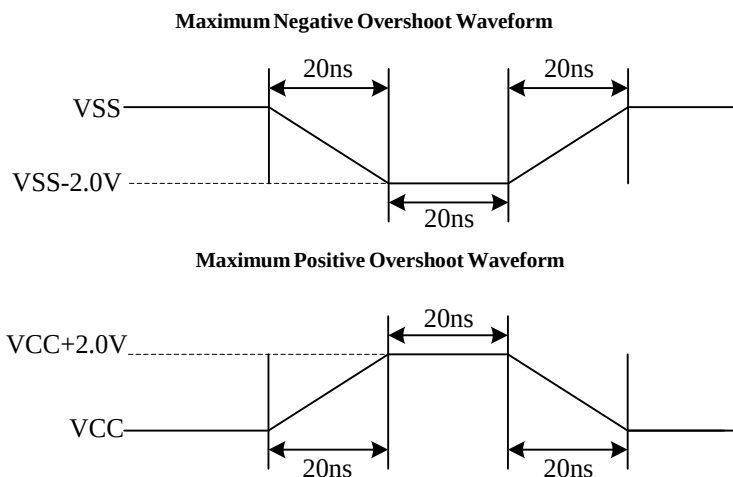
Figure 94. Input Test Waveform and Measurement Level
