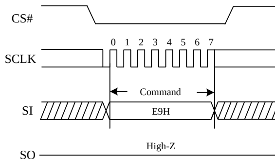
Figure 66. Disable 4-byte Mode Sequence Diagram (SPI)
