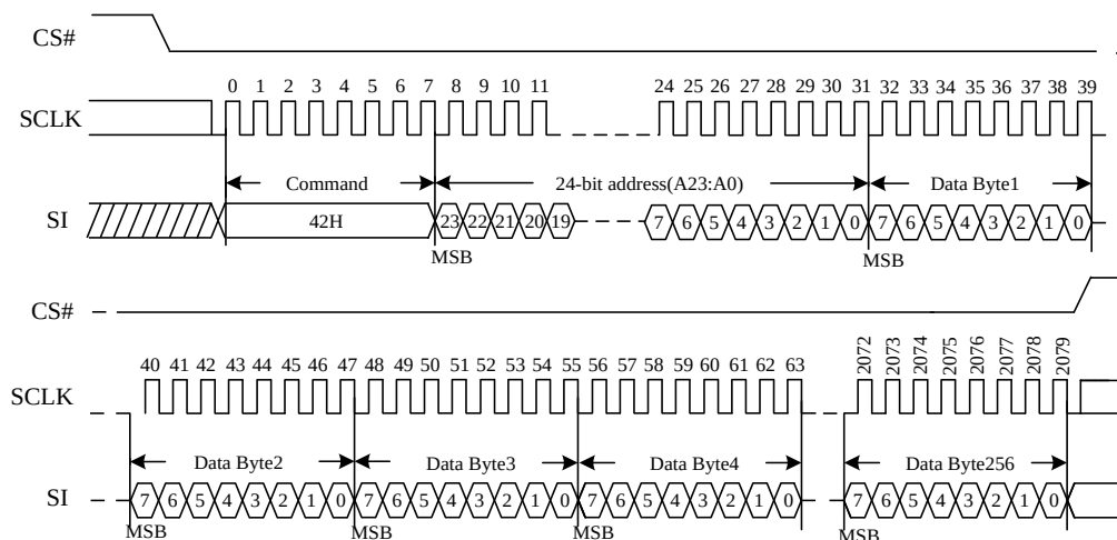
Figure 79. Program Security Registers command Sequence Diagram
