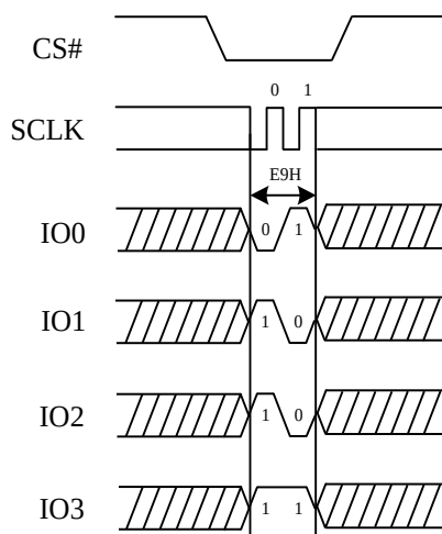
Figure 67. Disable 4-byte Mode Sequence Diagram (QPI)
