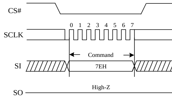
Figure 83. The Global Block/Sector Lock Sequence Diagram
