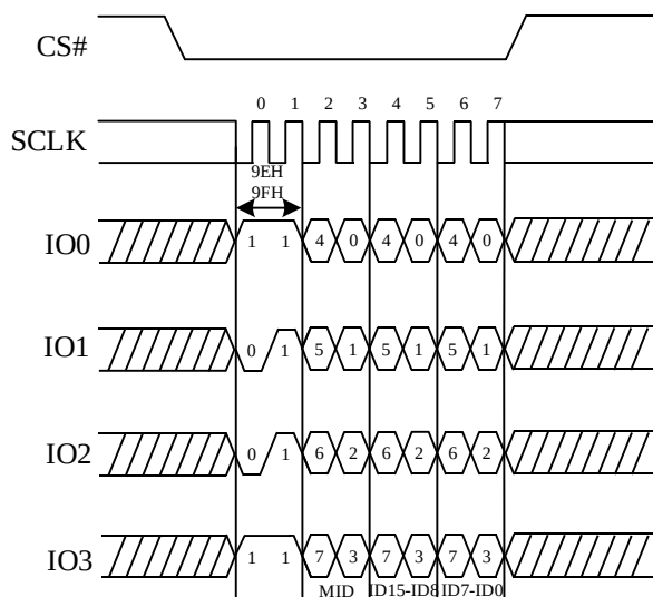
Figure 16. Read Identification ID Sequence Diagram (QPI)
