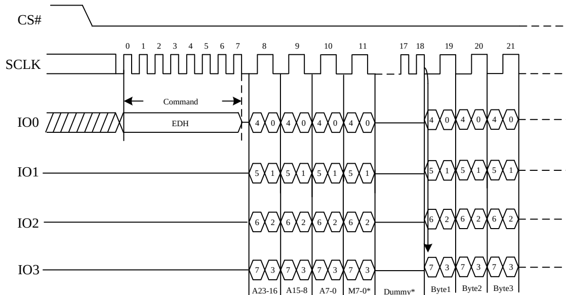
Figure 32. DTR Fast Read Quad I/O (Initial instruction or previous M5-4≠10, SPI Mode)
