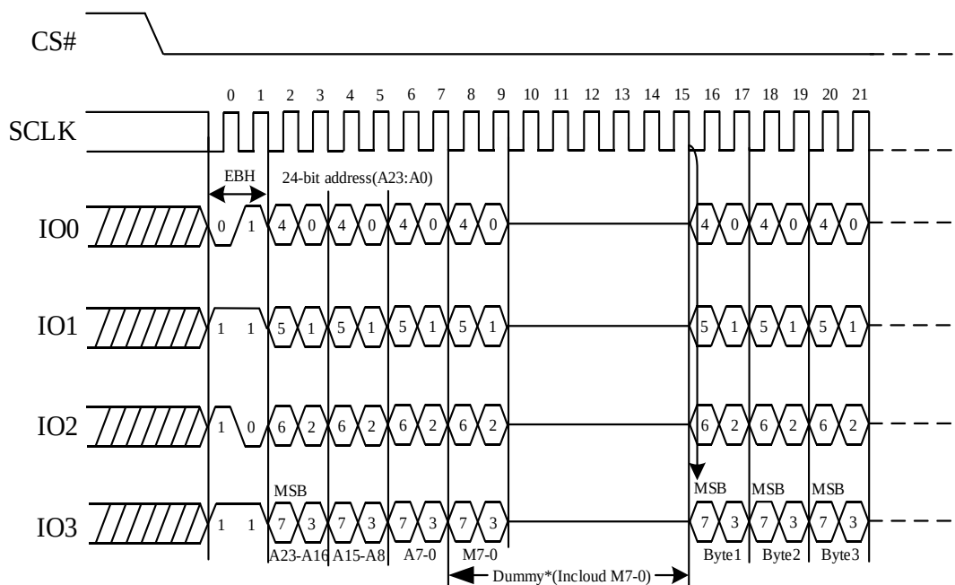
Figure 26. Quad I/O Fast Read Sequence Diagram (M5-4= (1, 0) QPI)
