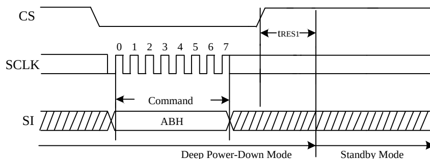
Figure 72. Release Power-Down Sequence Diagram
