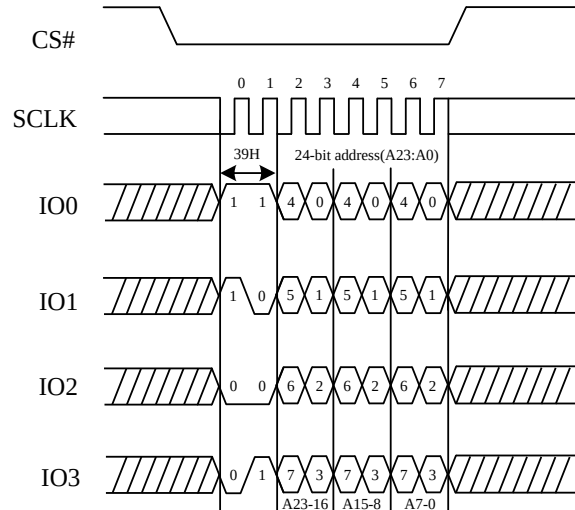
Figure 90. Individual Block/Sector Unlock command Sequence Diagram (QPI)
