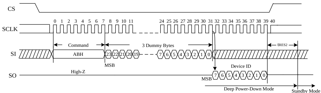
Figure 74. Release From Deep Power-Down/Read Device ID Sequence Diagram
