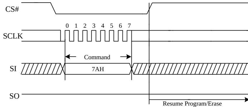
Figure 58. Program/Erase Resume Sequence Diagram
