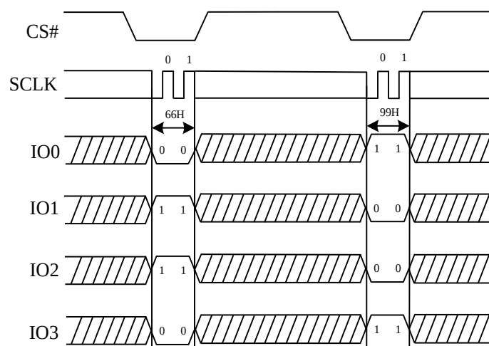
Figure 49. Enable Reset and Reset command Sequence Diagram (QPI)
