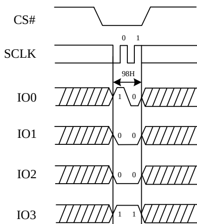
Figure 86. The Global Block/Sector Unlock Sequence Diagram (QPI)
