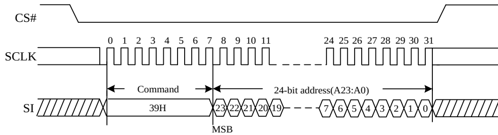
Figure 89. Individual Block/Sector Unlock command Sequence Diagram
