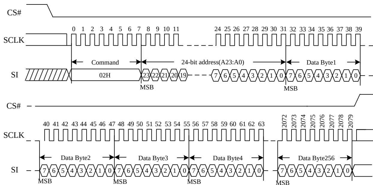
Figure 36. Page Program Sequence Diagram
