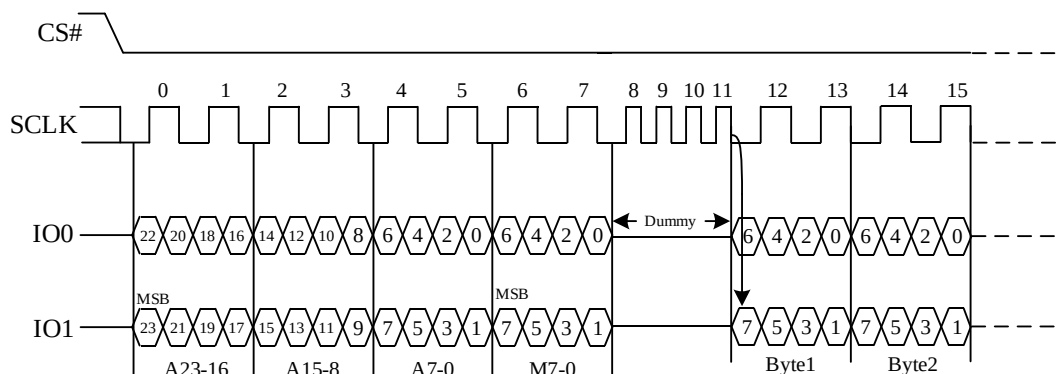
Figure 31. DTR Fast Read Dual I/O (Previous instruction set M5-4=10, SPI Mode only)
