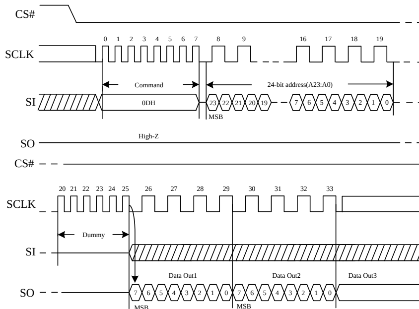
Figure 28. DTR Fast Read Instruction
