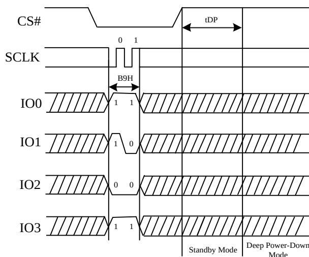
Figure 71. Deep Power-Down Sequence Diagram (QPI)
