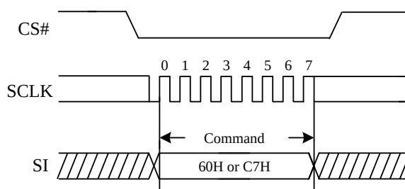
Figure 46. Chip Erase Sequence Diagram
