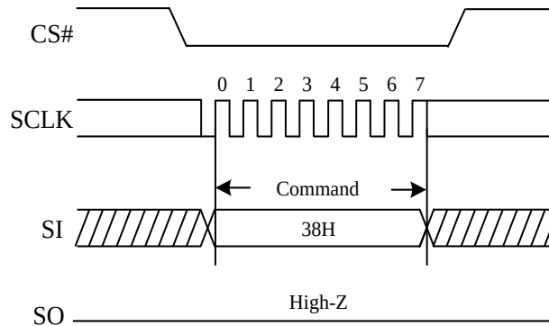
Figure 60. Enable QPI mode command Sequence Diagram
