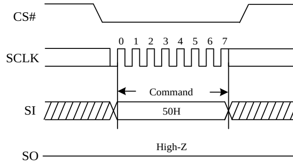
Figure 52. Write Enable for Volatile Status Register Sequence Diagram
