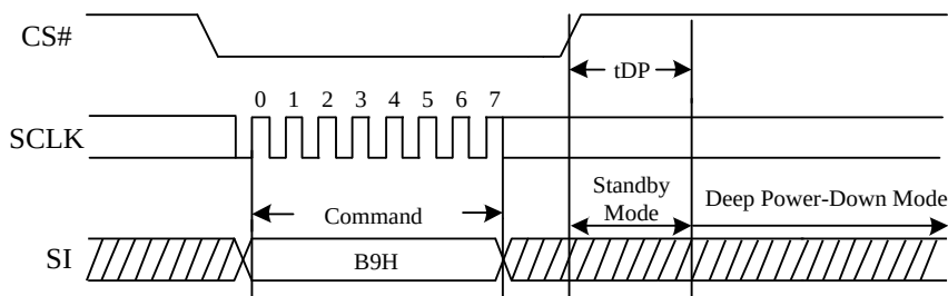
Figure 70. Deep Power-Down Sequence Diagram
