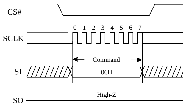
Figure 50. Write Enable Sequence Diagram
