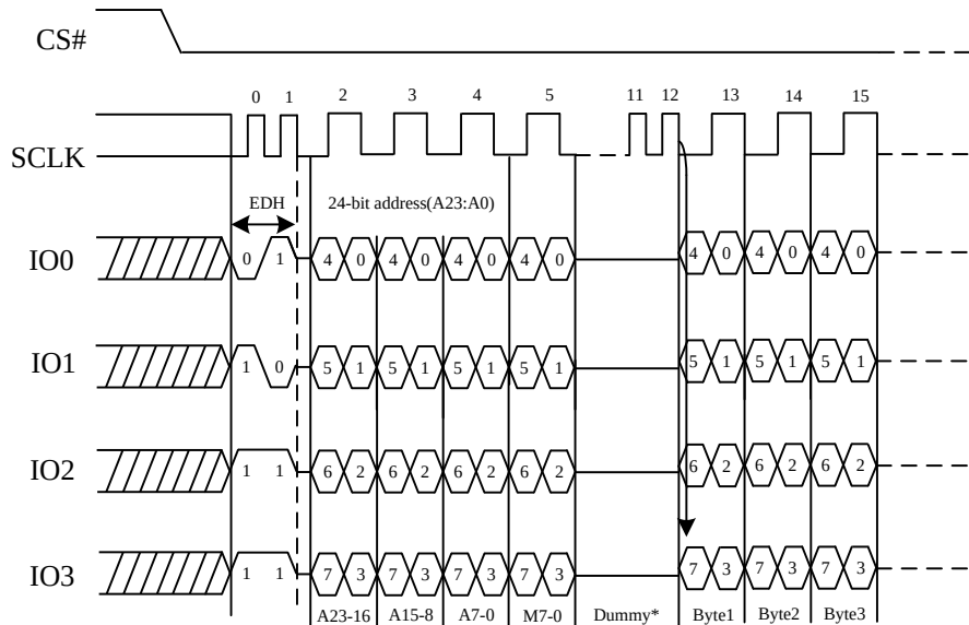
Figure 34. DTR Fast Read Quad I/O (Initial instruction or previous M5-4#10, QPI Mode)
