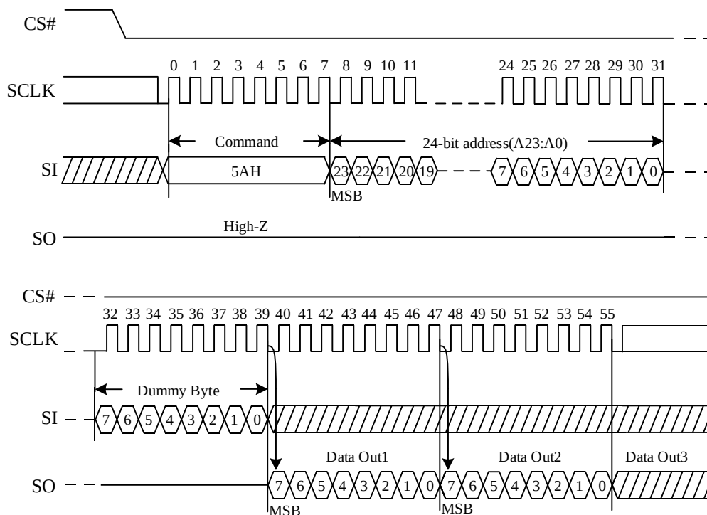
Figure 11. Read Serial Flash Discoverable Parameter command Sequence Diagram
