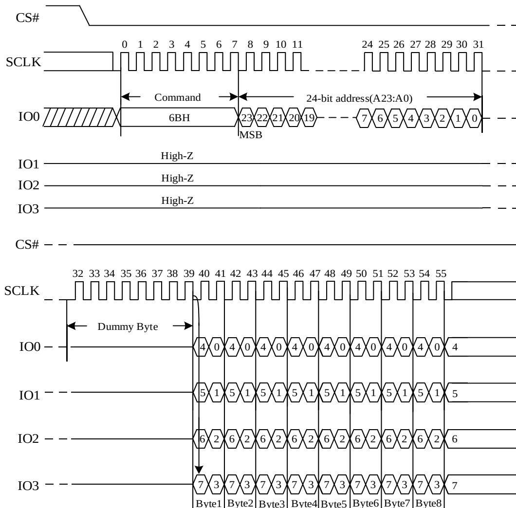
Figure 23. Quad Output Fast Read Sequence Diagram
