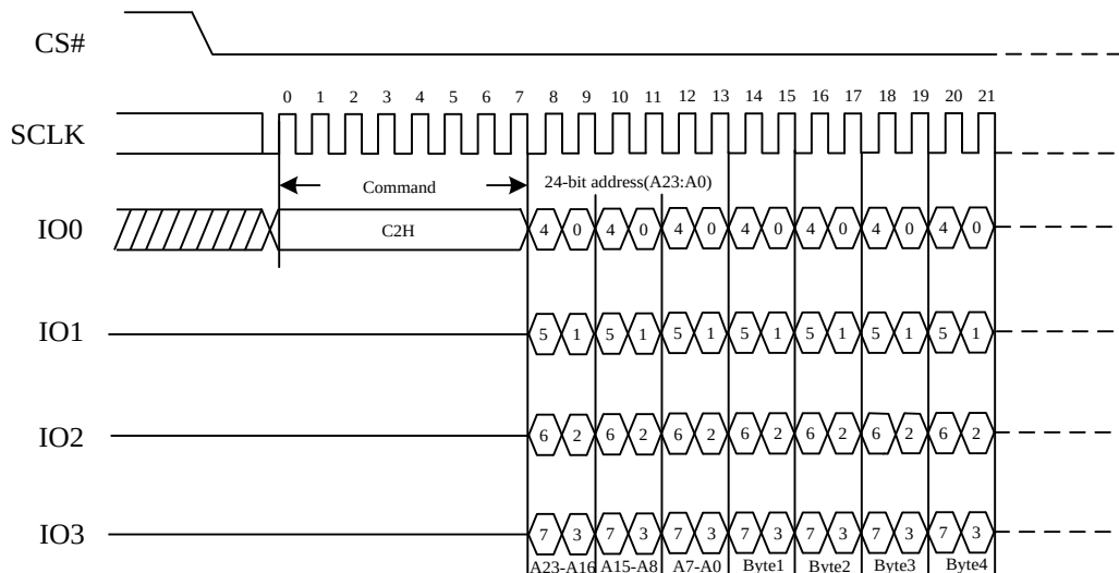
Figure 39. Quad Page Program Sequence Diagram
