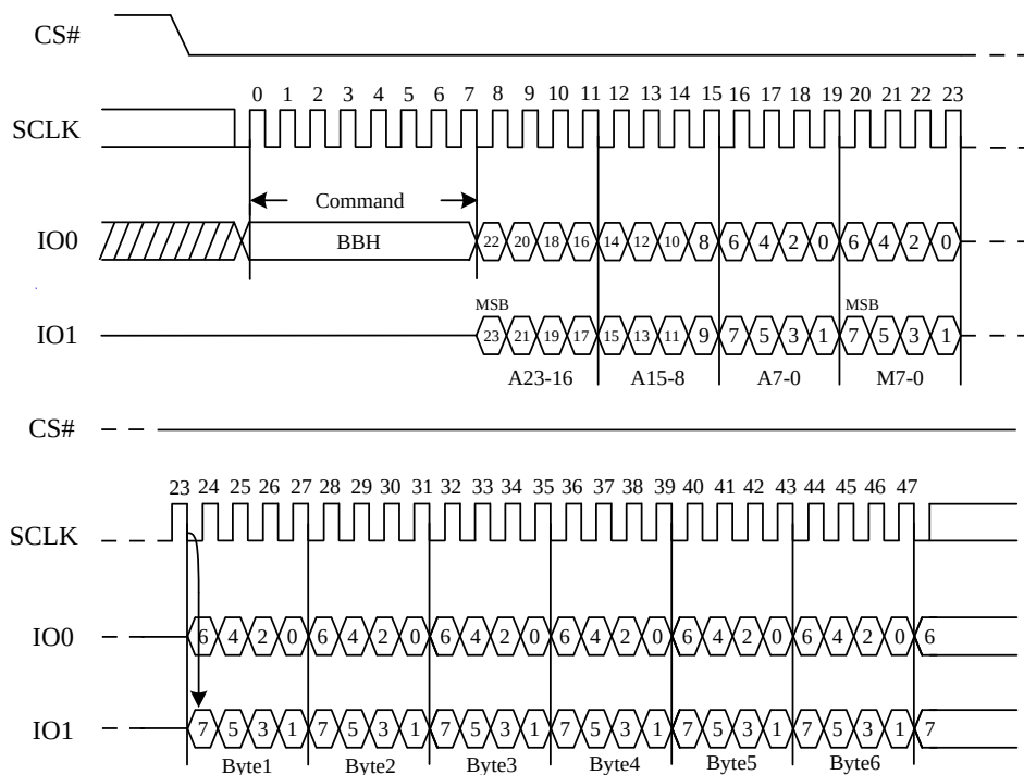
Figure 21. Dual I/O Fast Read Sequence Diagram (M5-4≠(1,0))
