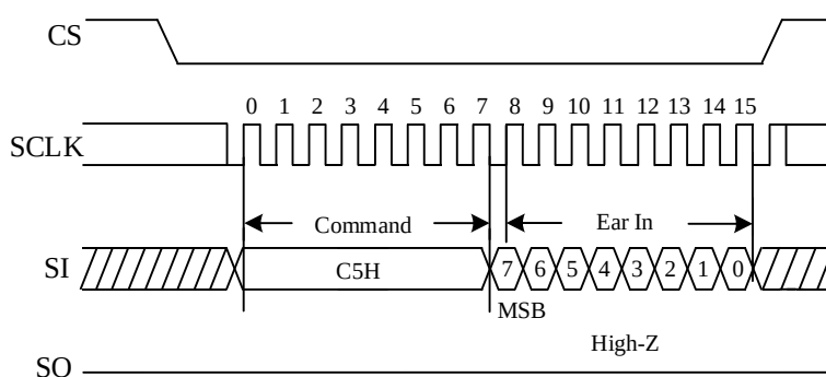
Figure 7. Write Extended Address Register Diagram
