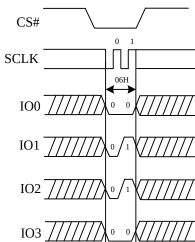
Figure 51. Write Enable Sequence Diagram (QPI)
