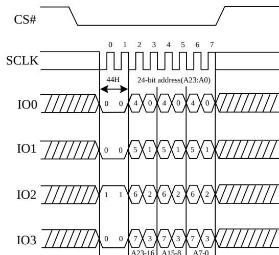
Figure 78. Erase Security Registers command Sequence Diagram (QPI)
