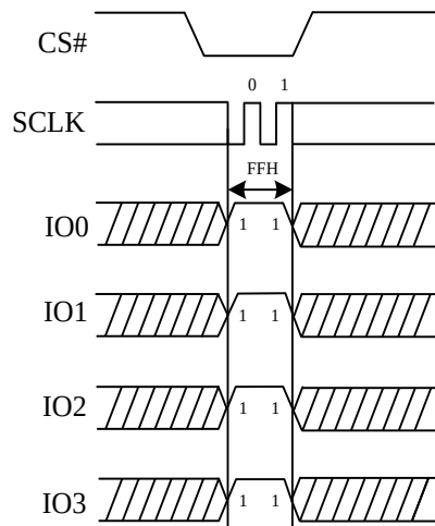
Figure 61. Disable QPI mode command Sequence Diagram (QPI)
