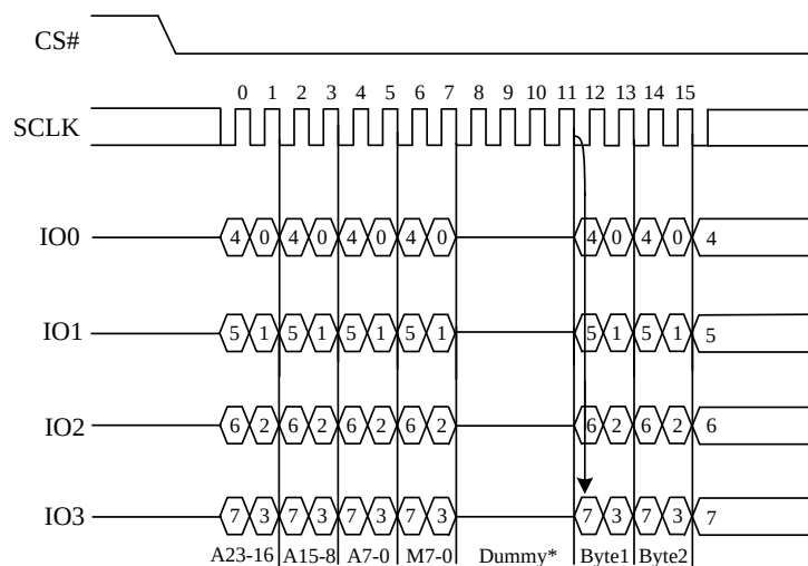
Figure 25. Quad I/O Fast Read Sequence Diagram (M5-4=(1,0))
