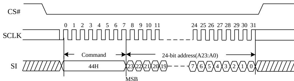
Figure 77. Erase Security Registers command Sequence Diagram
