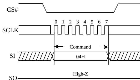
Figure 54. Write Disable Sequence Diagram
