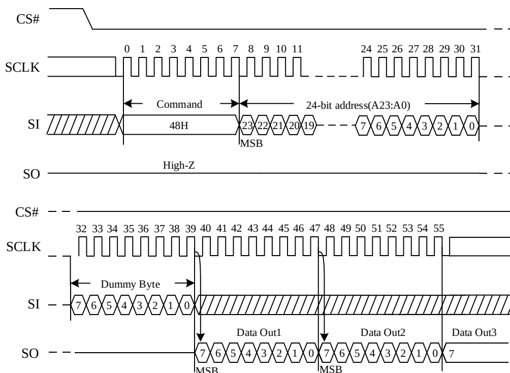
Figure 81. Read Security Registers command Sequence Diagram
