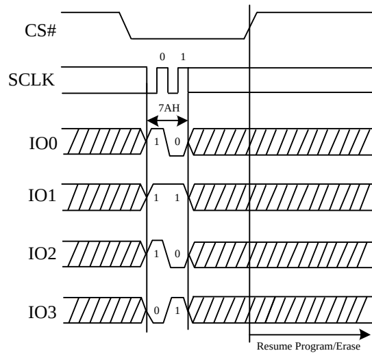
Figure 59. Program/Erase Resume Sequence Diagram (QPI)
