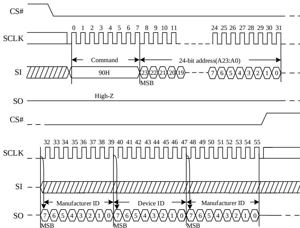
Figure 9. Read Manufacture ID/ Device ID Sequence Diagram
