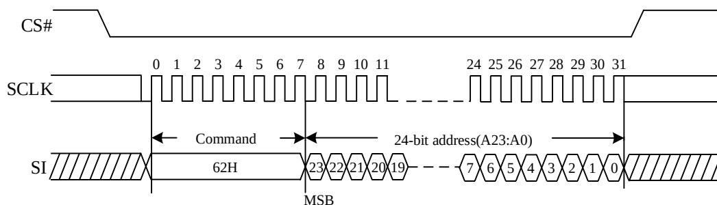
Figure 76. Program Strong Sequence Diagram
