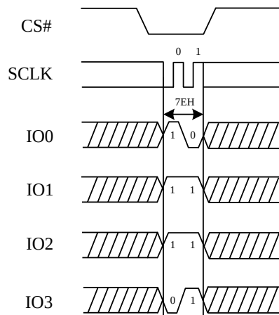
Figure 84. The Global Block/Sector Lock Sequence Diagram (QPI)
