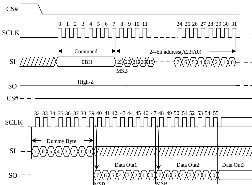
Figure 18. Read Data Bytes at Higher Speed Sequence Diagram
