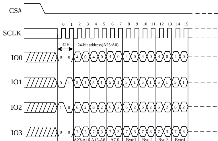
Figure 80. Program Security Registers command Sequence Diagram (QPI)
