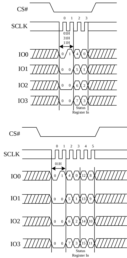
Figure 4. Write Status Register Sequence Diagram (QPI)
