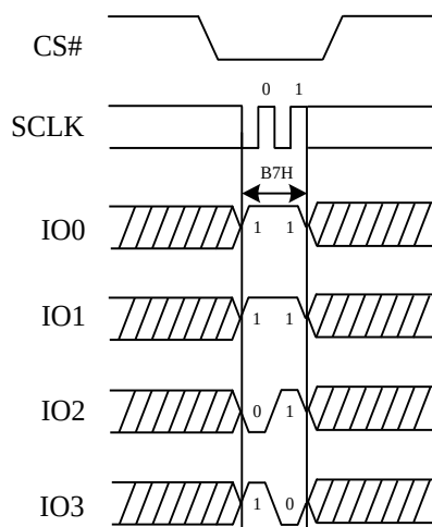
Figure 65. Enable 4-byte Mode Sequence Diagram (QPI)
