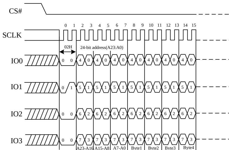
Figure 37. Page Program Sequence Diagram (QPI)
