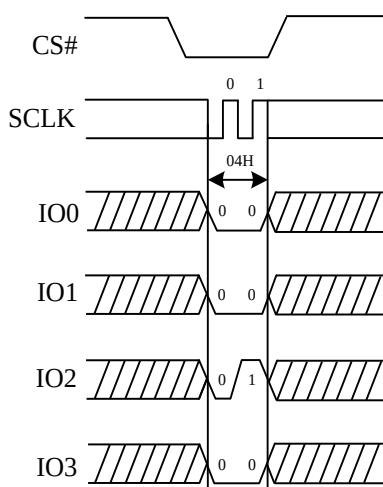
Figure 55. Write Disable Sequence Diagram (QPI)
