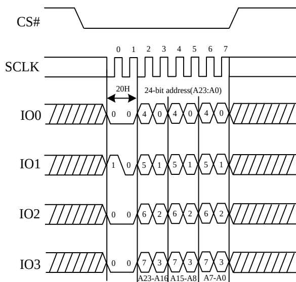
Figure 41. Sector Erase Sequence Diagram (QPI)
