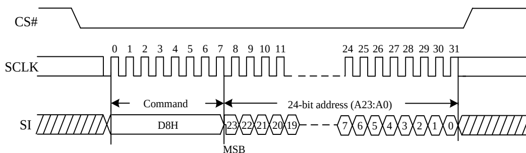
Figure 44. 64KB Block Erase Sequence Diagram
