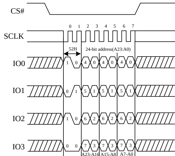
Figure 43. 32KB Block Erase Sequence Diagram (QPI)
