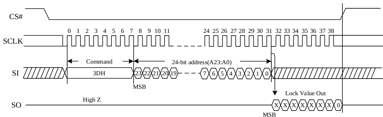
Figure 91. Read Individual Block/Sector lock command Sequence Diagram
