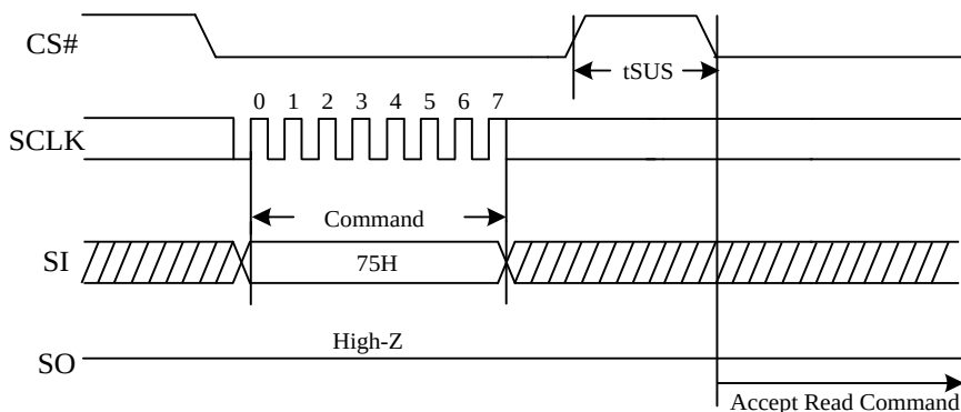
Figure 56. Program/Erase Suspend Sequence Diagram
