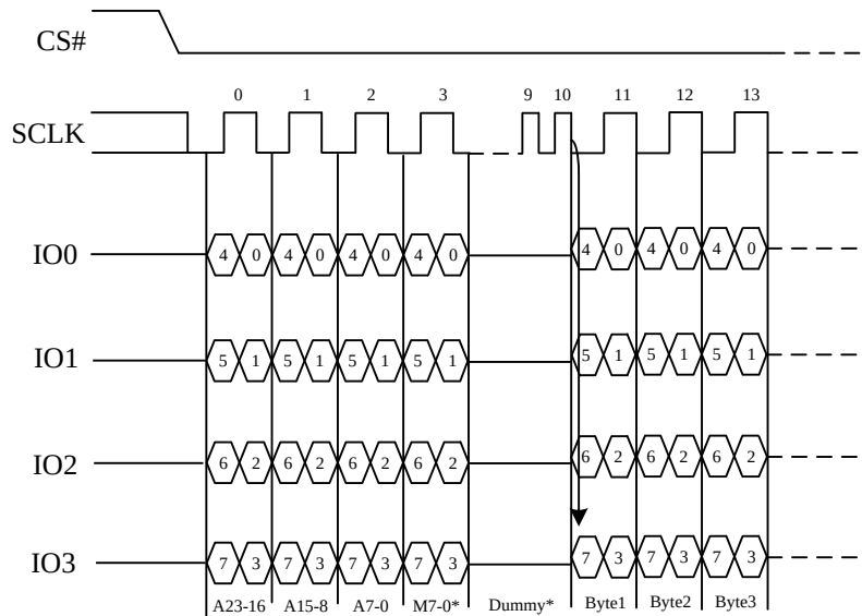
Figure 33. DTR Fast Read Quad I/O (Previous instruction set M5-4=10, SPI Mode)
