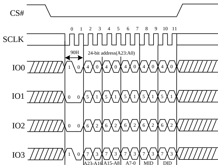
Figure 10. Read Manufacture ID/ Device ID Sequence Diagram (QPI)
