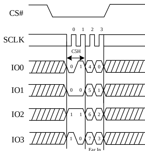
Figure 8. Write Extended Address Register Diagram (QPI)
