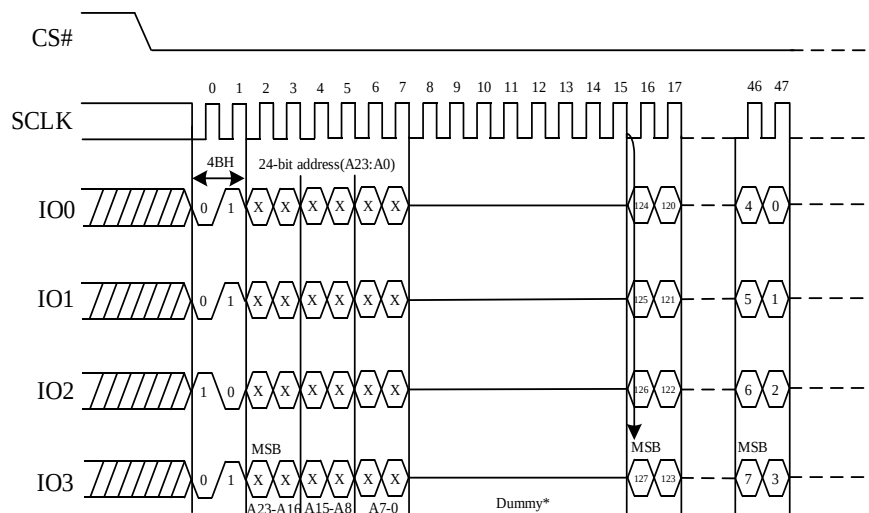
Figure 14. Read Unique ID (RUID) Sequence (QPI)
