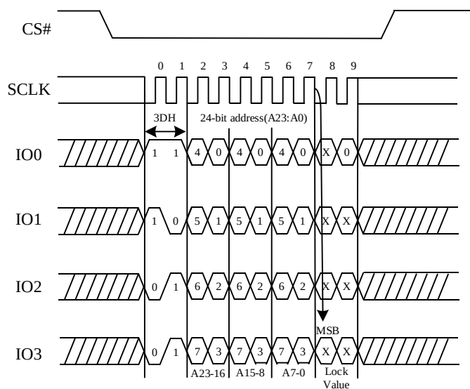
Figure 92. Read Individual Block/Sector lock command Sequence Diagram (QPI)
