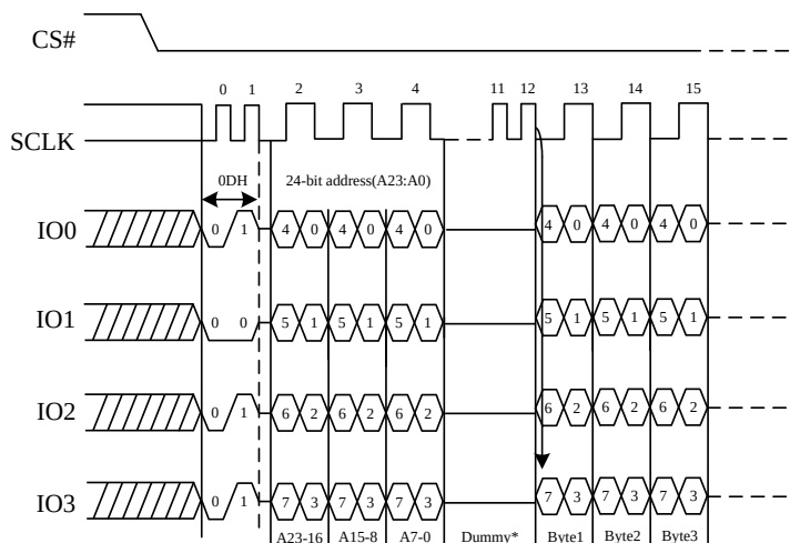
Figure 29. DTR Fast Read Instruction (QPI)
