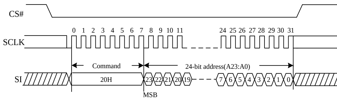
Figure 40. Sector Erase Sequence Diagram
