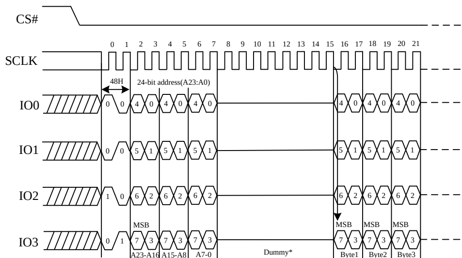
Figure 82. Read Security Registers command Sequence Diagram (QPI)
