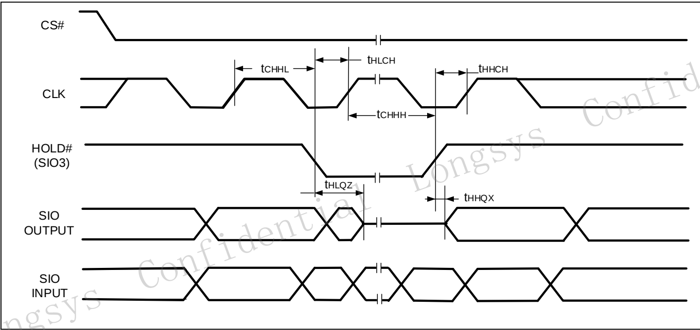
Figure 35 HOLD# Timing
