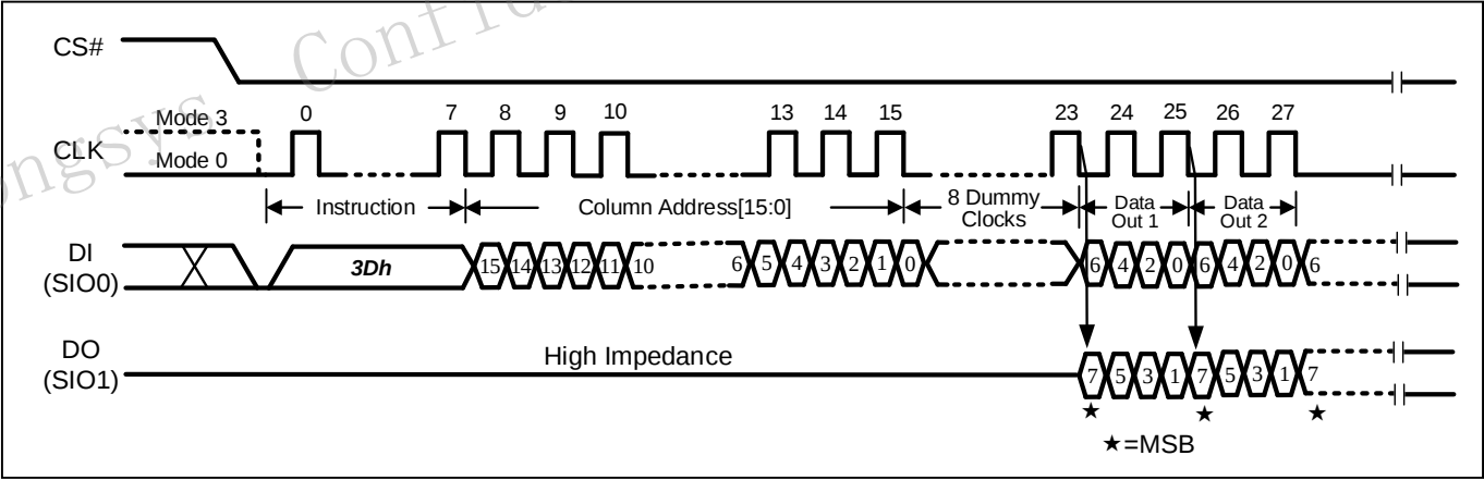
Figure 20 DTR Read Dual Output (3Dh) Sequence
