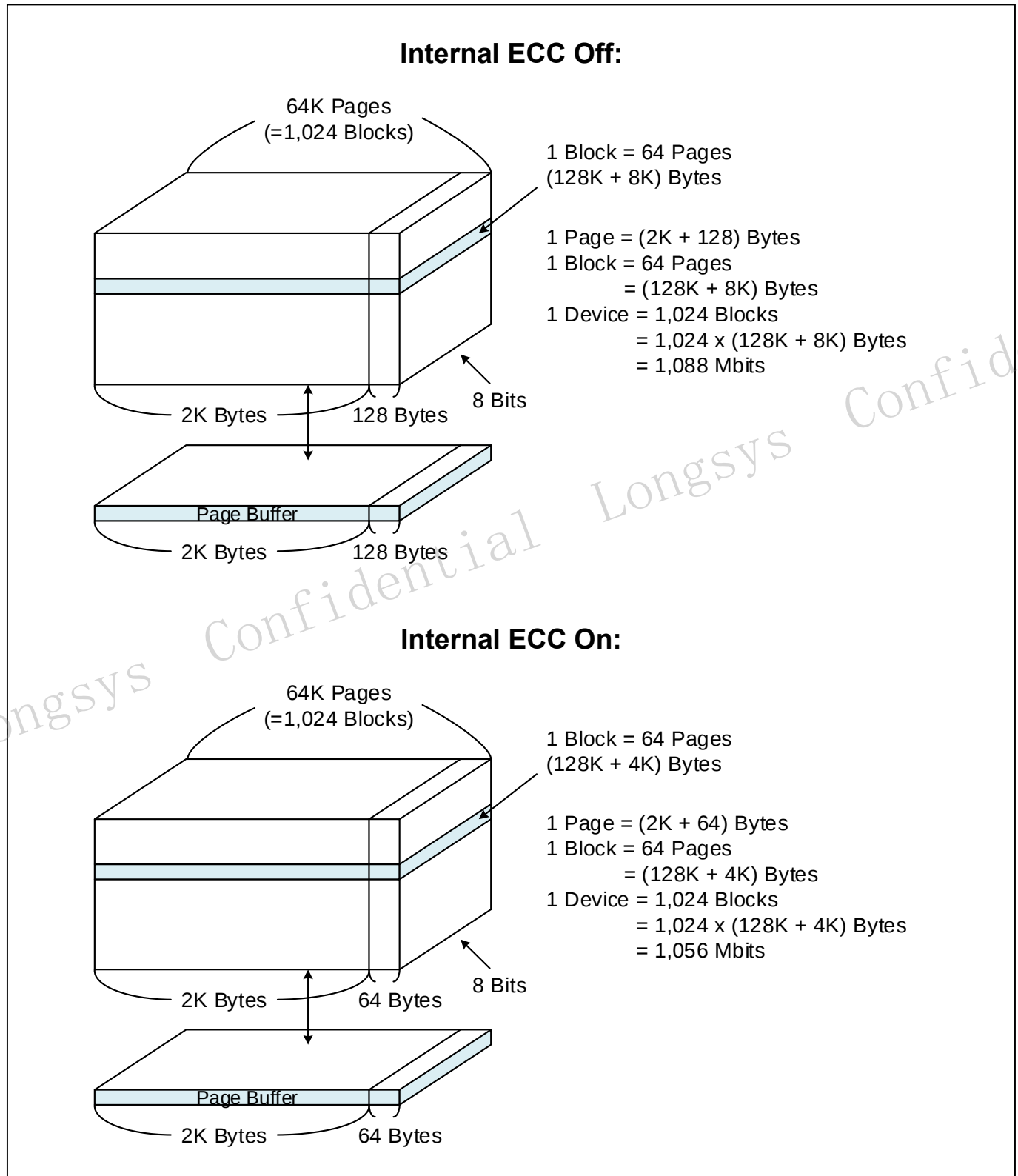
Figure 4 Array Organization
