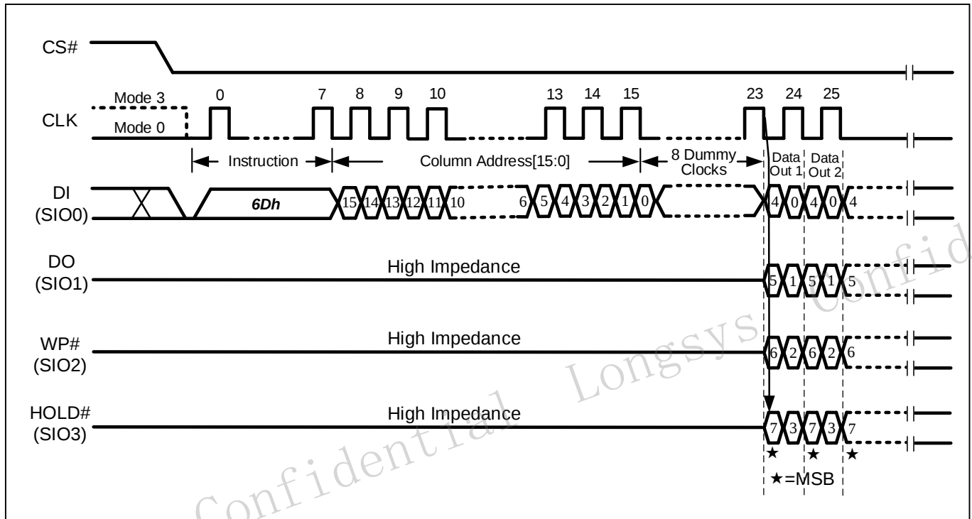
Figure 21 DTR Read Quad Output (6Dh) Sequence
