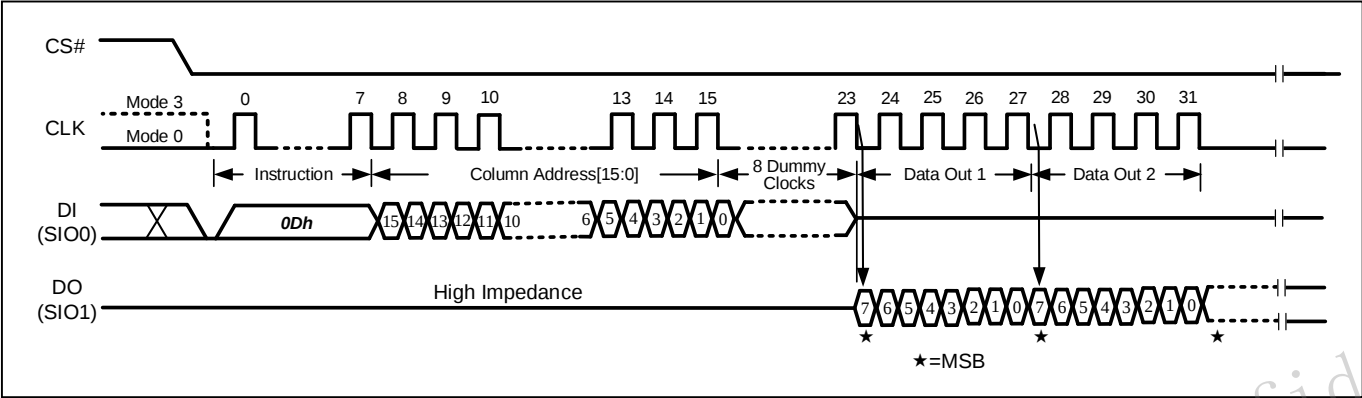
Figure 19 DTR Read (0Dh) Sequence
