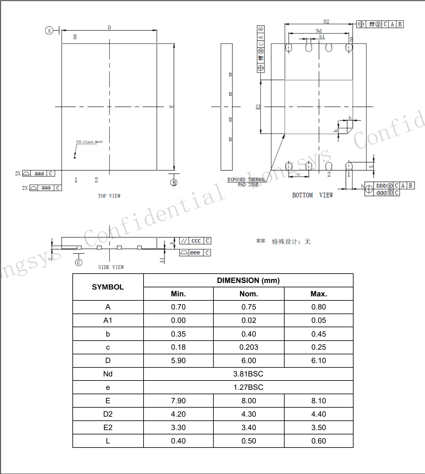
Figure 37 8-WSON (6x8mm) Package Information
