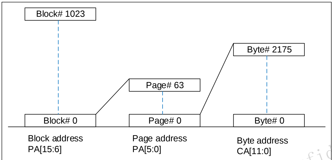
Figure 5 Address Mapping
