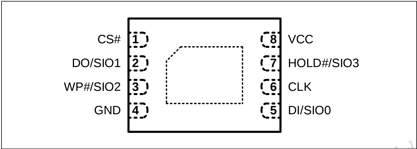
Figure 2 Pin Configuration 8-WSON
