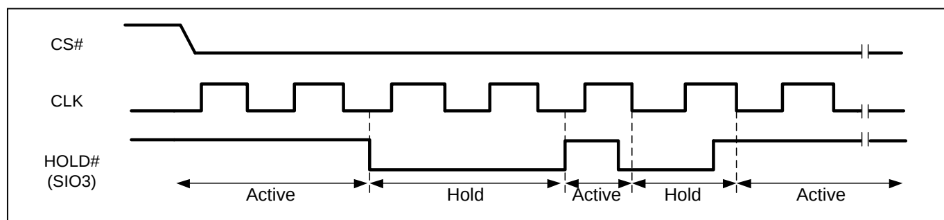
Figure 7 Hold Condition
