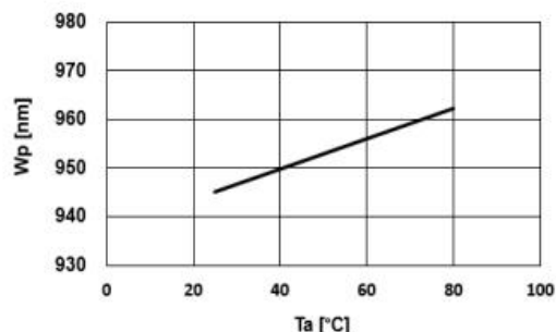
Fig.5— Peak Wavelength (@1000mA) vs. Ambient Temperature
