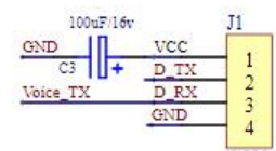
Downloader port
