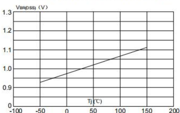
Fig6 Normalized Breakdown Voltage vs. Tj
