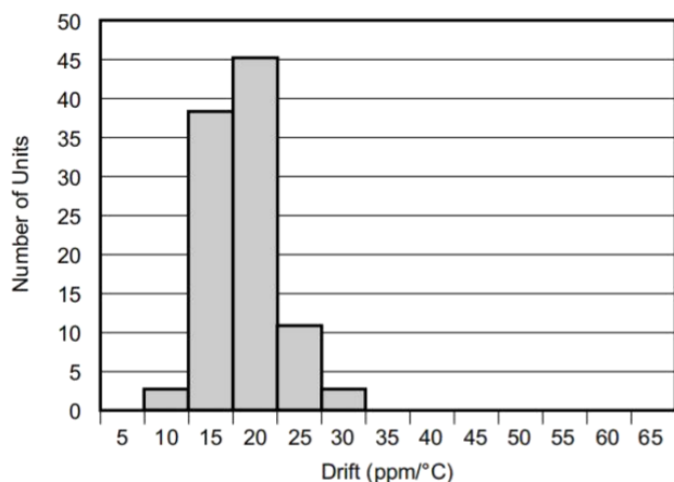
Figure 1. Temperature Drift (0°C to 70°C)
