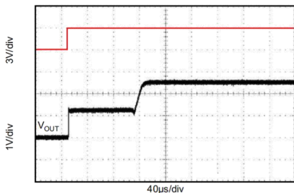
Figure 13. Step Response, C_L = 0 , 3-V Start-Up
