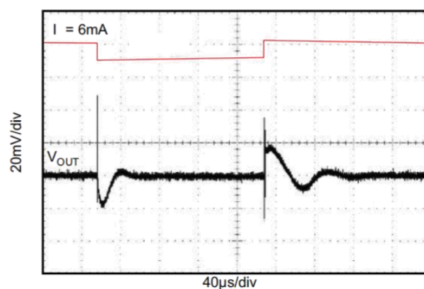
Figure 18. 1 to 6-mA Load Transient ( C_L = 1 \mu F )
