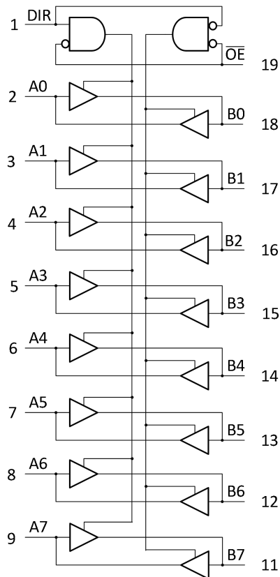
Fig. 1. Logic symbol
