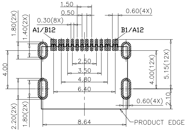
RECOMMENDED PCB LAYOUT(COMPONENT SIDE) TOLERANCE FOR PCB LAYOUT IS \pm 0.05
