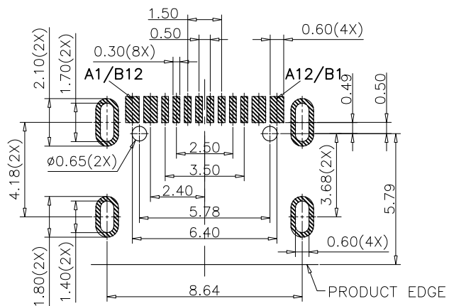
RECOMMENDED PCB LAYOUT(COMPONENT SIDE) TOLERANCE FOR PCB LAYOUT IS \pm 0.05
