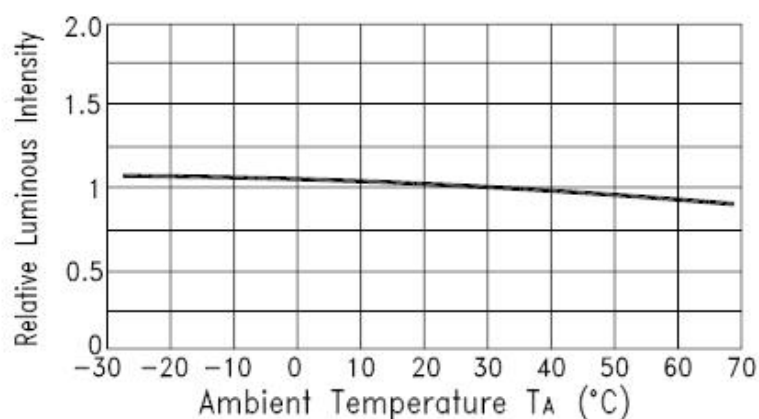
Fig.5 Luminous Intensity vs. Ambient Temperature
