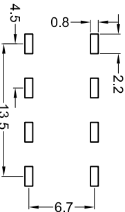
PCB LAYOUT
