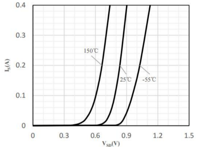
Body-Diode Characteristics
