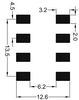
PCB LAYOUT
