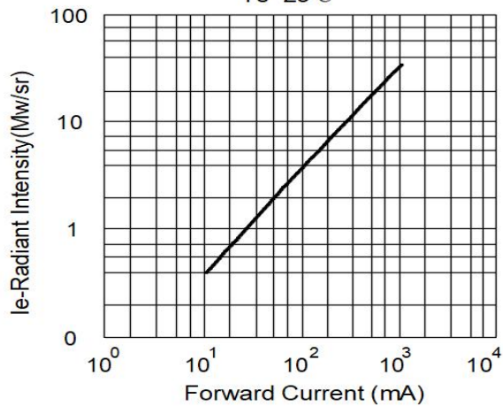
Radiant Intensity vs. Forward Current Ts=25°C
