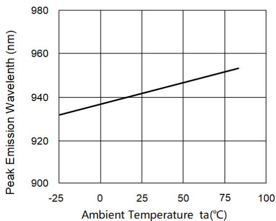
Peak Emission Wavelength Vs. Ambient Temperature
