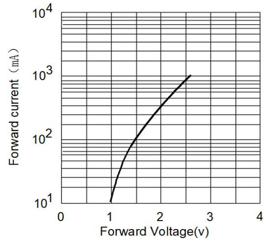
Forward current VS Forward Voltage(v) Ts=25°C
