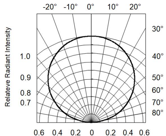
Relative Radiant Intensity vs. Angular Displacement
