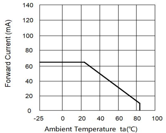
Forward Current Vs Temperature Ts=25°C
