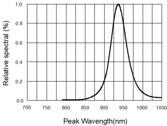
Relative spectral Vs peak Wavelength(nm) Ts=25°C
