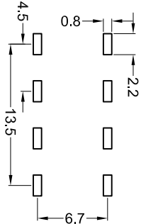
PCB LAYOUT
